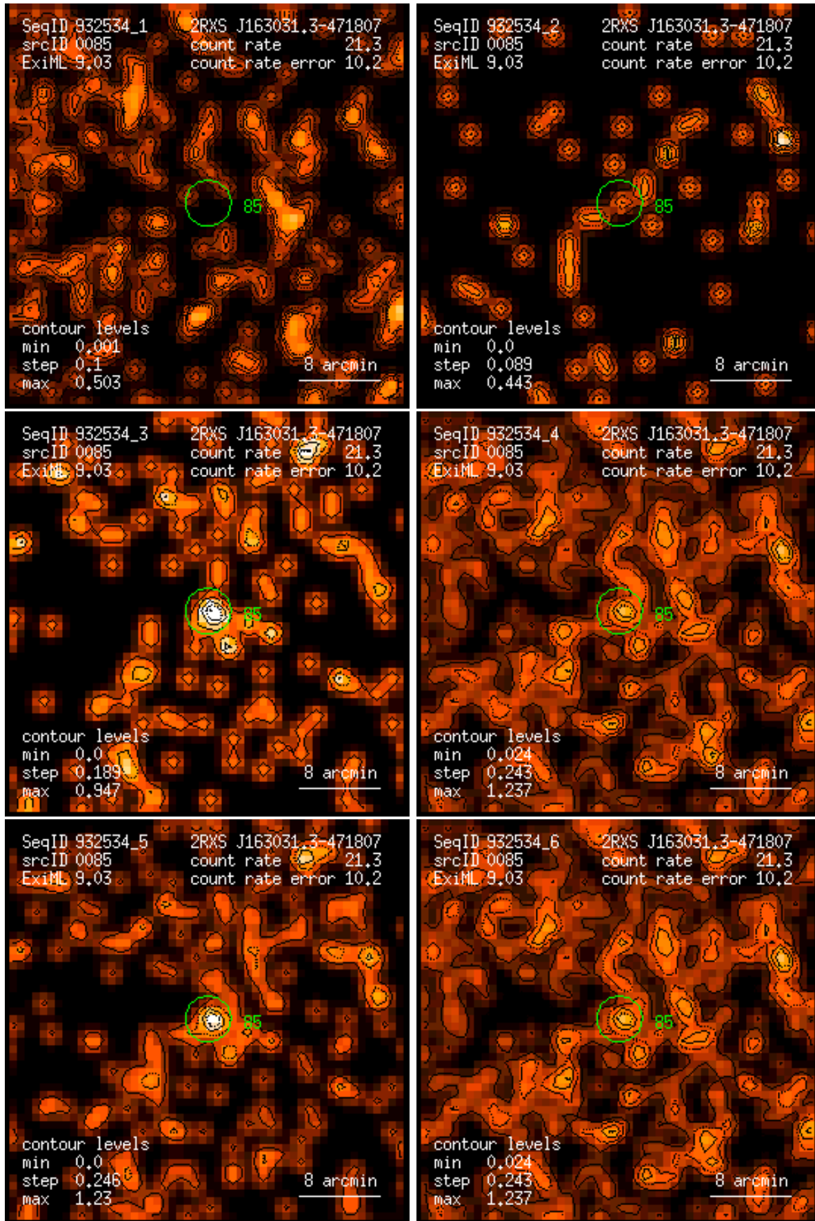
Figure 85: RASS 932534: detection 0085: band rate images, Gaussian filter: (1) PSPC channels 11 – 41, (2) 52 – 90, (3) 91 – 201, (4) 11 – 235, (5) 52 – 201, (6) 11 – 201. Broad band rates in counts/ks. Band rate contour levels in counts/ks/arcmin 2 .
