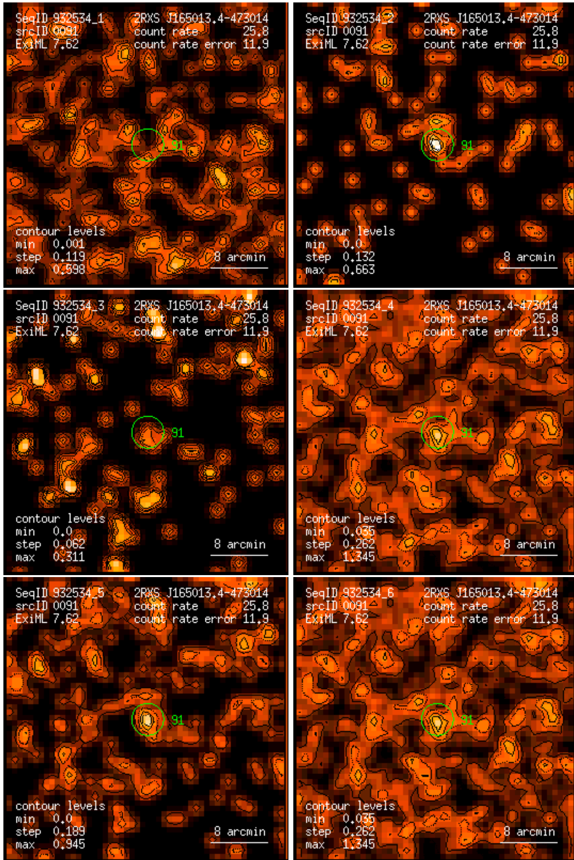
Figure 91: RASS 932534: detection 0091: band rate images, Gaussian filter: (1) PSPC channels 11 – 41, (2) 52 – 90, (3) 91 – 201, (4) 11 – 235, (5) 52 – 201, (6) 11 – 201. Broad band rates in counts/ks. Band rate contour levels in counts/ks/arcmin 2 .
