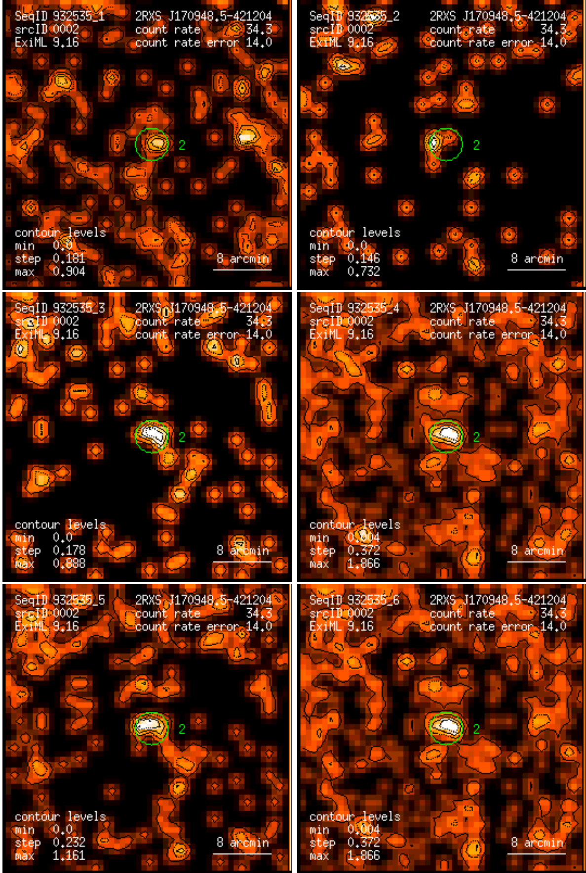
Figure 2: RASS 932535: detection 0002: band rate images, Gaussian filter: (1) PSPC channels 11 – 41, (2) 52 – 90, (3) 91 – 201, (4) 11 – 235, (5) 52 – 201, (6) 11 – 201. Broad band rates in counts/ks. Band rate contour levels in counts/ks/arcmin 2 .
