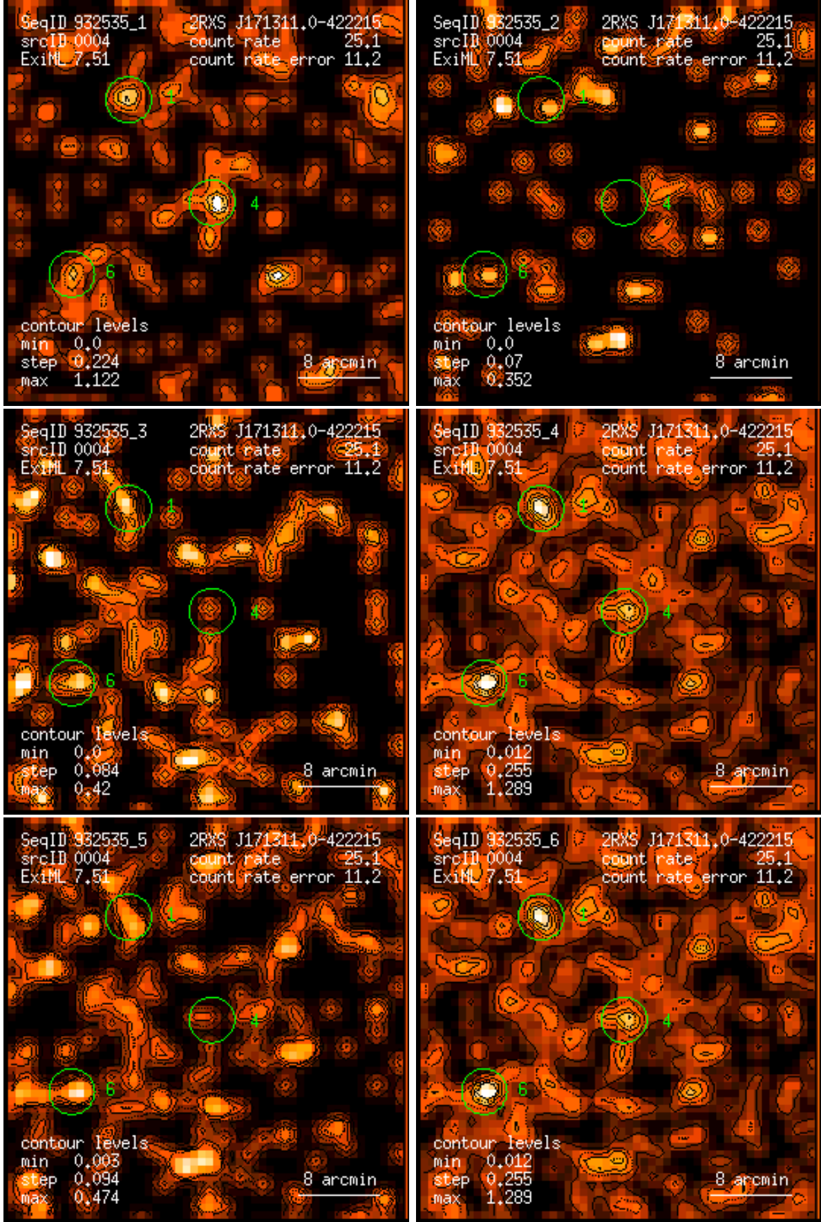
Figure 4: RASS 932535: detection 0004: band rate images, Gaussian filter: (1) PSPC channels 11 – 41, (2) 52 – 90, (3) 91 – 201, (4) 11 – 235, (5) 52 – 201, (6) 11 – 201. Broad band rates in counts/ks. Band rate contour levels in counts/ks/arcmin 2 .
