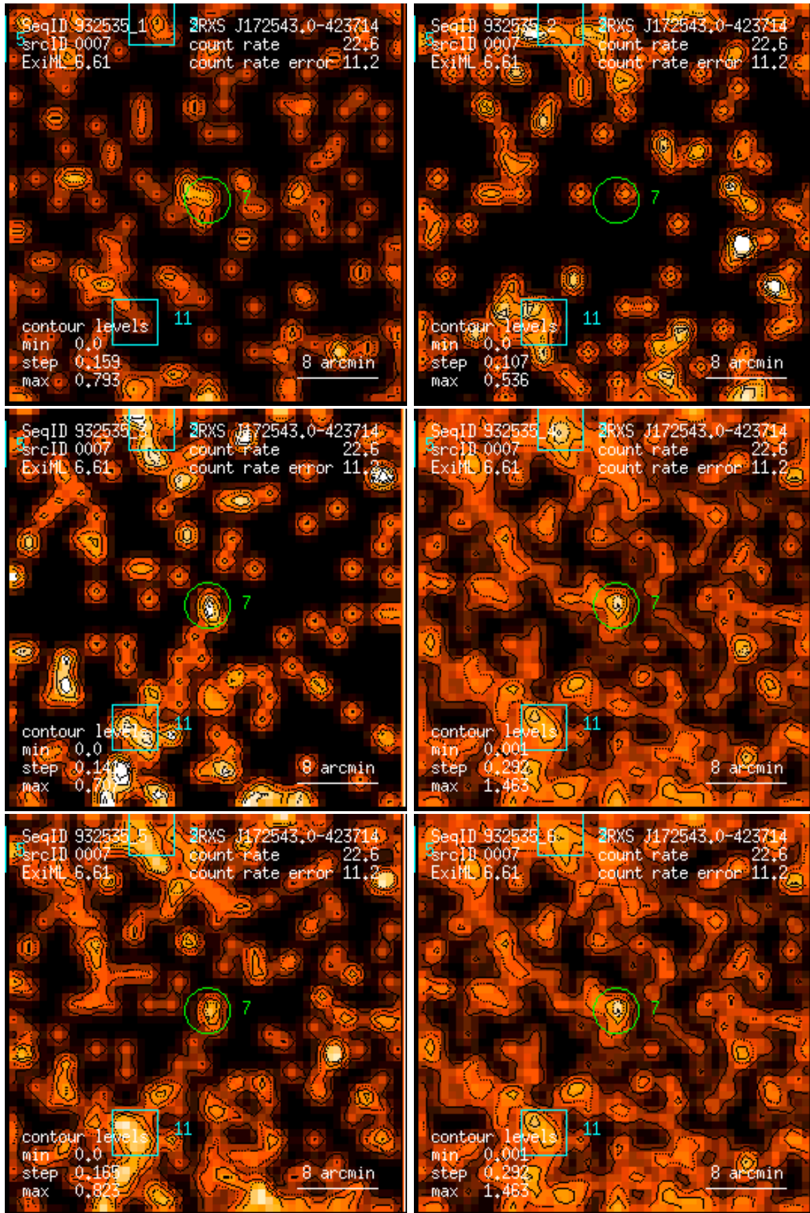
Figure 7: RASS 932535: detection 0007: band rate images, Gaussian filter: (1) PSPC channels 11 – 41, (2) 52 – 90, (3) 91 – 201, (4) 11 – 235, (5) 52 – 201, (6) 11 – 201. Broad band rates in counts/ks. Band rate contour levels in counts/ks/arcmin 2 .
