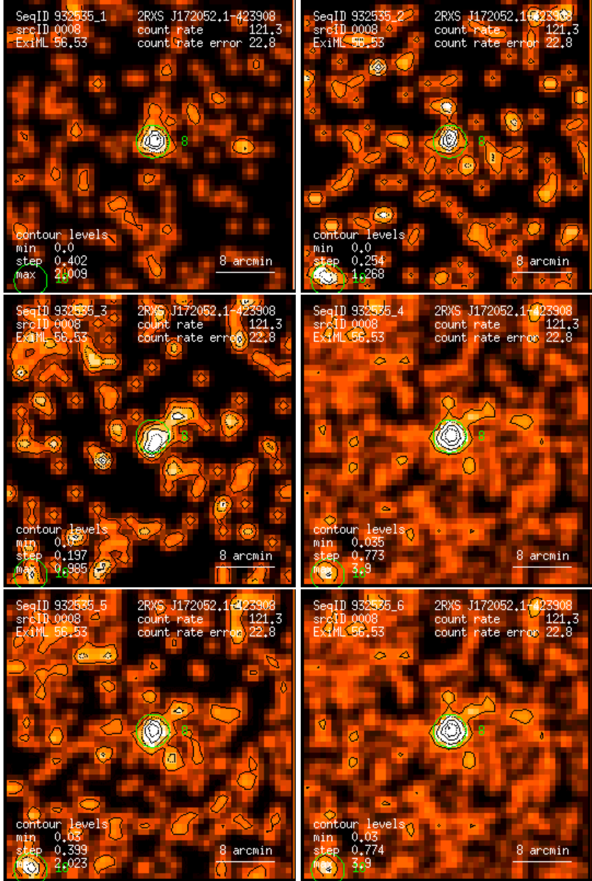
Figure 8: RASS 932535: detection 0008: band rate images, Gaussian filter: (1) PSPC channels 11 – 41, (2) 52 – 90, (3) 91 – 201, (4) 11 – 235, (5) 52 – 201, (6) 11 – 201. Broad band rates in counts/ks. Band rate contour levels in counts/ks/arcmin 2 .
