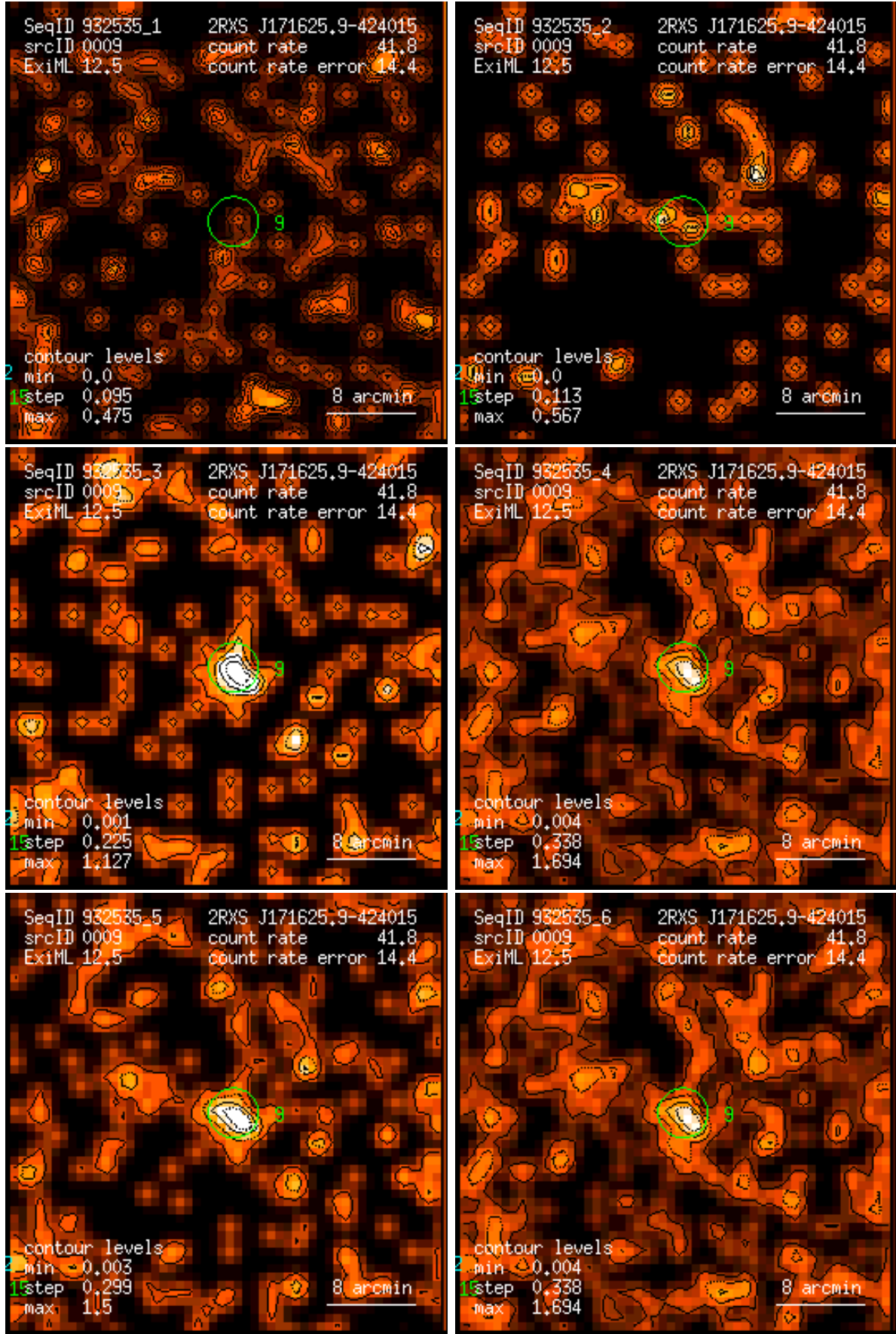
Figure 9: RASS 932535: detection 0009: band rate images, Gaussian filter: (1) PSPC channels 11 – 41, (2) 52 – 90, (3) 91 – 201, (4) 11 – 235, (5) 52 – 201, (6) 11 – 201. Broad band rates in counts/ks. Band rate contour levels in counts/ks/arcmin 2 .
