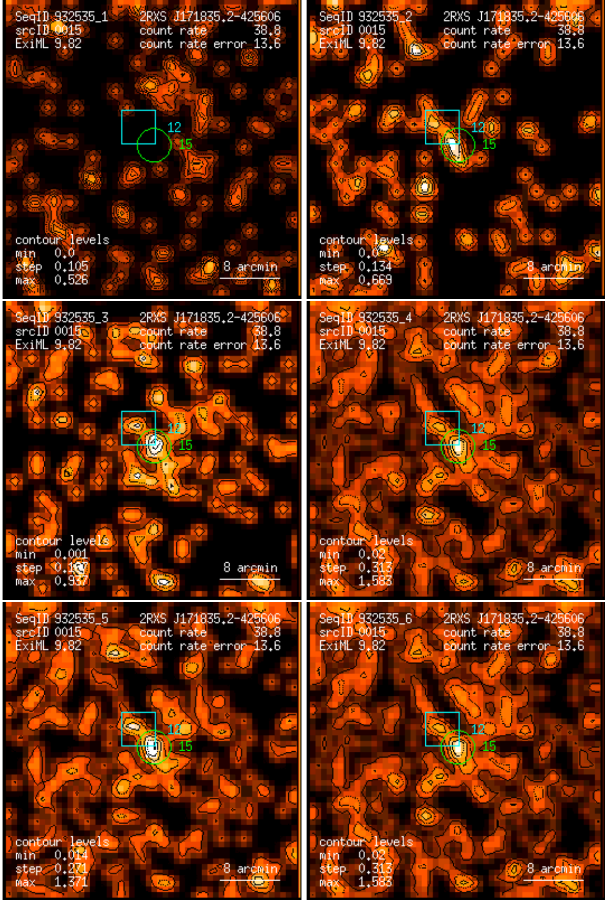
Figure 15: RASS 932535: detection 0015: band rate images, Gaussian filter: (1) PSPC channels 11 – 41, (2) 52 – 90, (3) 91 – 201, (4) 11 – 235, (5) 52 – 201, (6) 11 – 201. Broad band rates in counts/ks. Band rate contour levels in counts/ks/arcmin 2 .
