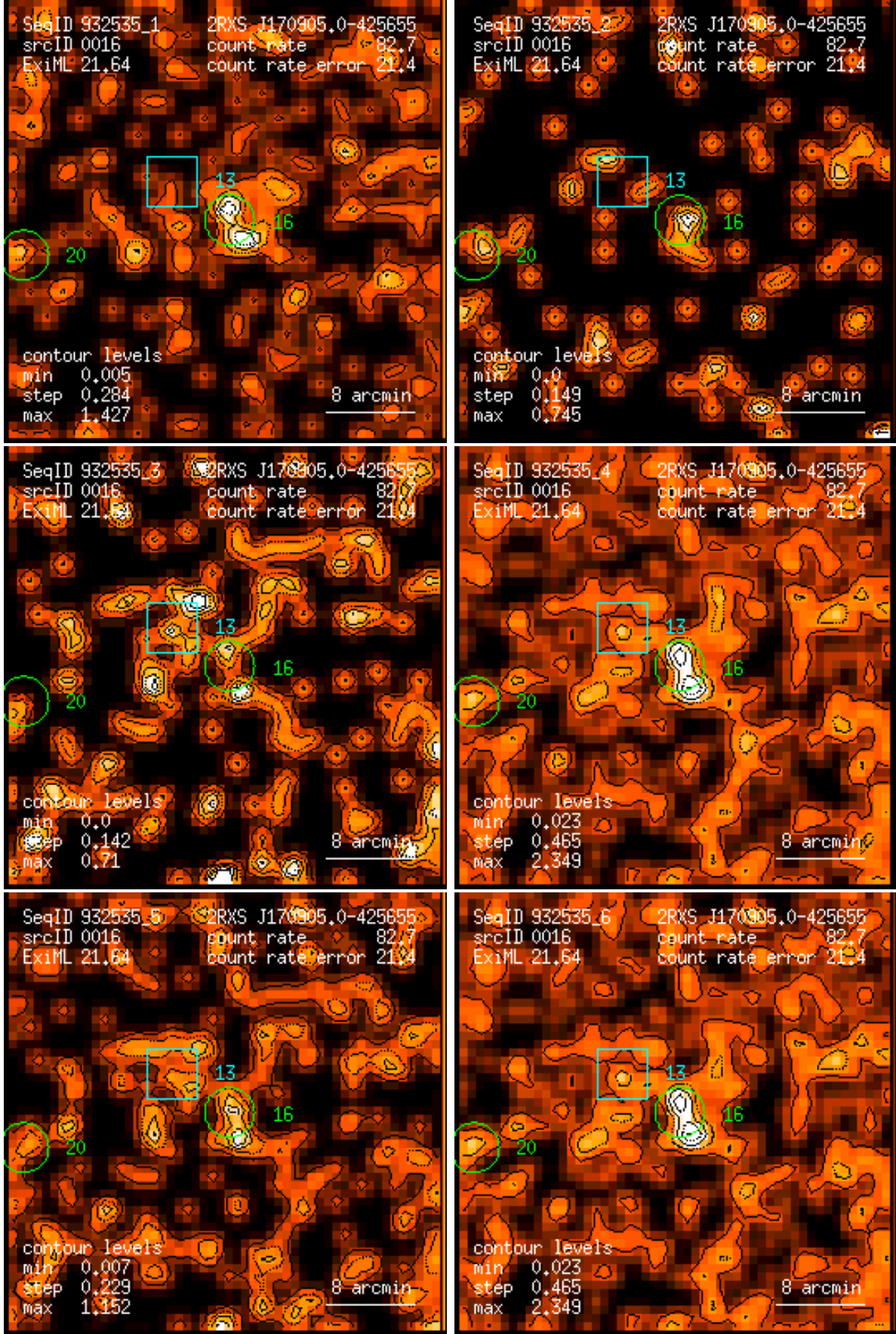
Figure 16: RASS 932535: detection 0016: band rate images, Gaussian filter: (1) PSPC channels 11 – 41, (2) 52 – 90, (3) 91 – 201, (4) 11 – 235, (5) 52 – 201, (6) 11 – 201. Broad band rates in counts/ks. Band rate contour levels in counts/ks/arcmin 2 .
