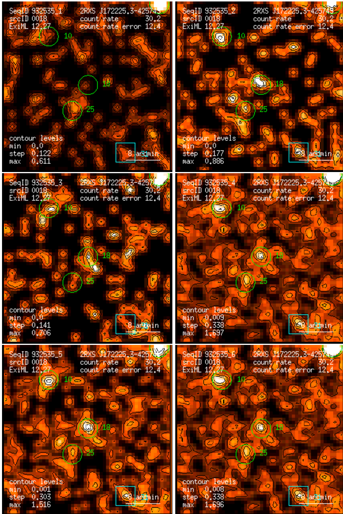
Figure 18: RASS 932535: detection 0018: band rate images, Gaussian filter: (1) PSPC channels 11 – 41, (2) 52 – 90, (3) 91 – 201, (4) 11 – 235, (5) 52 – 201, (6) 11 – 201. Broad band rates in counts/ks. Band rate contour levels in counts/ks/arcmin 2 .
