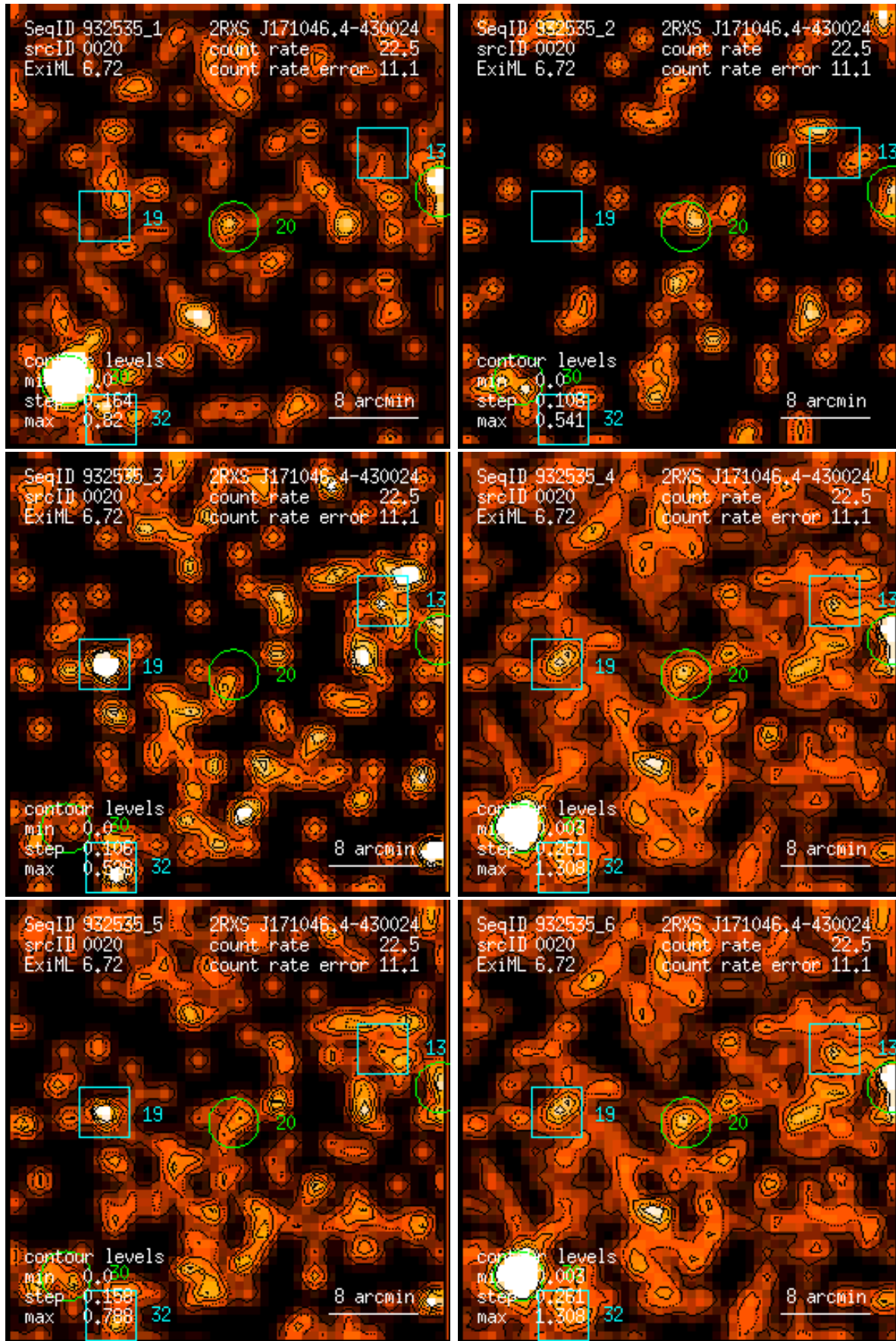
Figure 20: RASS 932535: detection 0020: band rate images, Gaussian filter: (1) PSPC channels 11 – 41, (2) 52 – 90, (3) 91 – 201, (4) 11 – 235, (5) 52 – 201, (6) 11 – 201. Broad band rates in counts/ks. Band rate contour levels in counts/ks/arcmin 2 .
