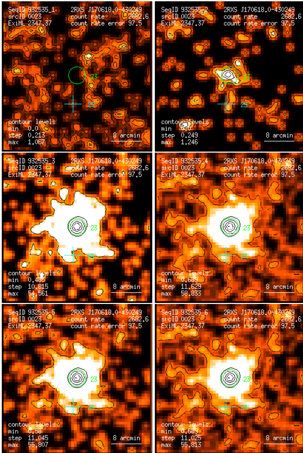
Figure 23: RASS 932535: detection 0023: band rate images, Gaussian filter: (1) PSPC channels 11 – 41, (2) 52 – 90, (3) 91 – 201, (4) 11 – 235, (5) 52 – 201, (6) 11 – 201. Broad band rates in counts/ks. Band rate contour levels in counts/ks/arcmin 2 .
