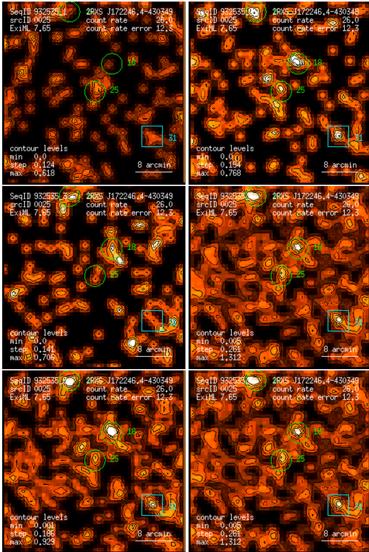
Figure 25: RASS 932535: detection 0025: band rate images, Gaussian filter: (1) PSPC channels 11 – 41, (2) 52 – 90, (3) 91 – 201, (4) 11 – 235, (5) 52 – 201, (6) 11 – 201. Broad band rates in counts/ks. Band rate contour levels in counts/ks/arcmin 2 .
