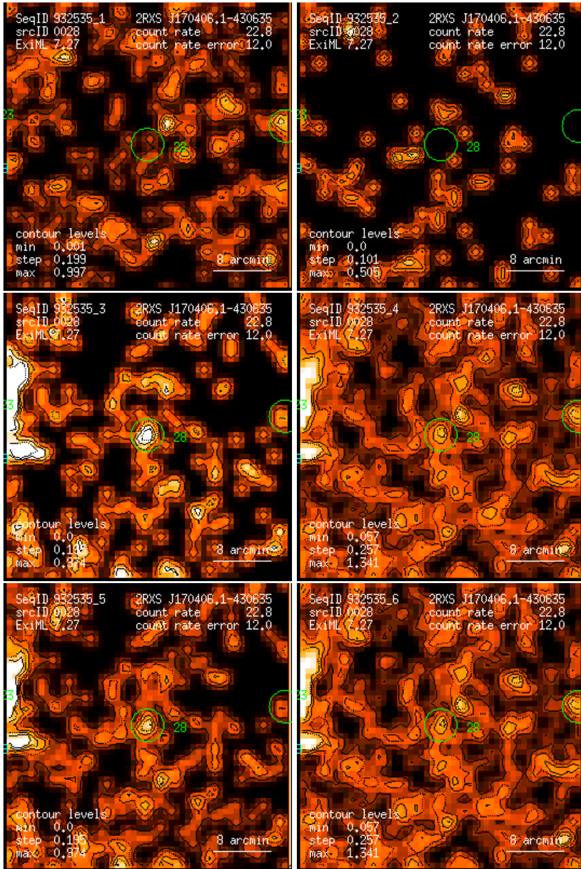
Figure 28: RASS 932535: detection 0028: band rate images, Gaussian filter: (1) PSPC channels 11 – 41, (2) 52 – 90, (3) 91 – 201, (4) 11 – 235, (5) 52 – 201, (6) 11 – 201. Broad band rates in counts/ks. Band rate contour levels in counts/ks/arcmin 2 .
