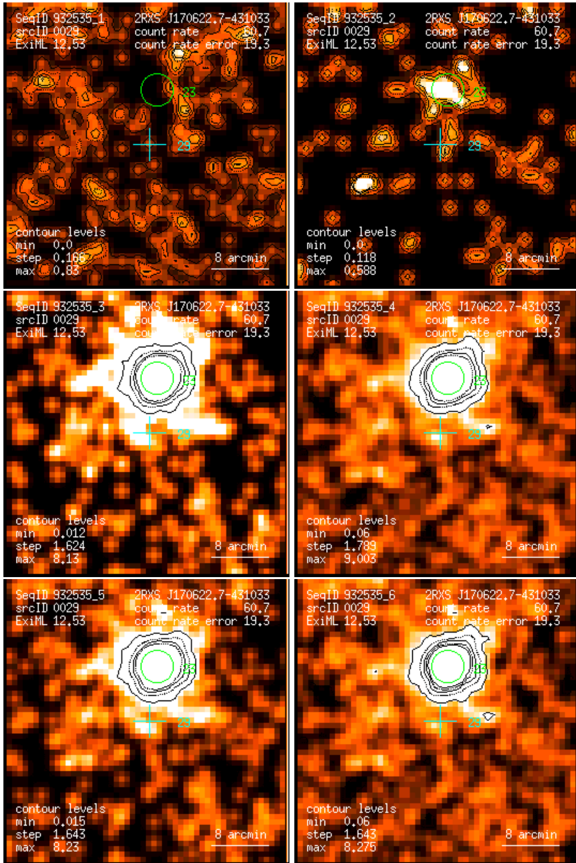
Figure 29: RASS 932535: detection 0029: band rate images, Gaussian filter: (1) PSPC channels 11 – 41, (2) 52 – 90, (3) 91 – 201, (4) 11 – 235, (5) 52 – 201, (6) 11 – 201. Broad band rates in counts/ks. Band rate contour levels in counts/ks/arcmin 2 .
