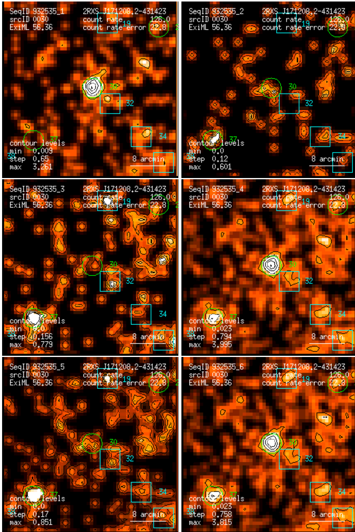
Figure 30: RASS 932535: detection 0030: band rate images, Gaussian filter: (1) PSPC channels 11 – 41, (2) 52 – 90, (3) 91 – 201, (4) 11 – 235, (5) 52 – 201, (6) 11 – 201. Broad band rates in counts/ks. Band rate contour levels in counts/ks/arcmin 2 .
