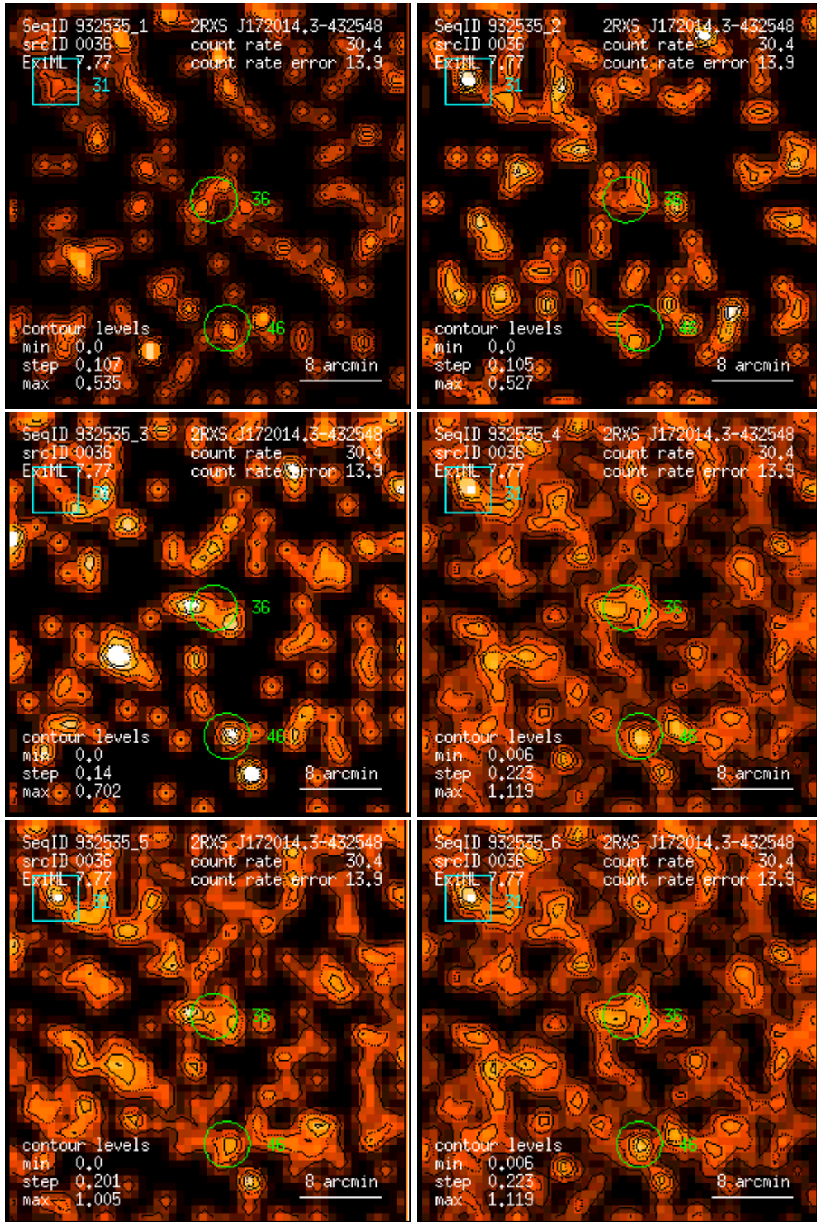
Figure 36: RASS 932535: detection 0036: band rate images, Gaussian filter: (1) PSPC channels 11 – 41, (2) 52 – 90, (3) 91 – 201, (4) 11 – 235, (5) 52 – 201, (6) 11 – 201. Broad band rates in counts/ks. Band rate contour levels in counts/ks/arcmin 2 .
