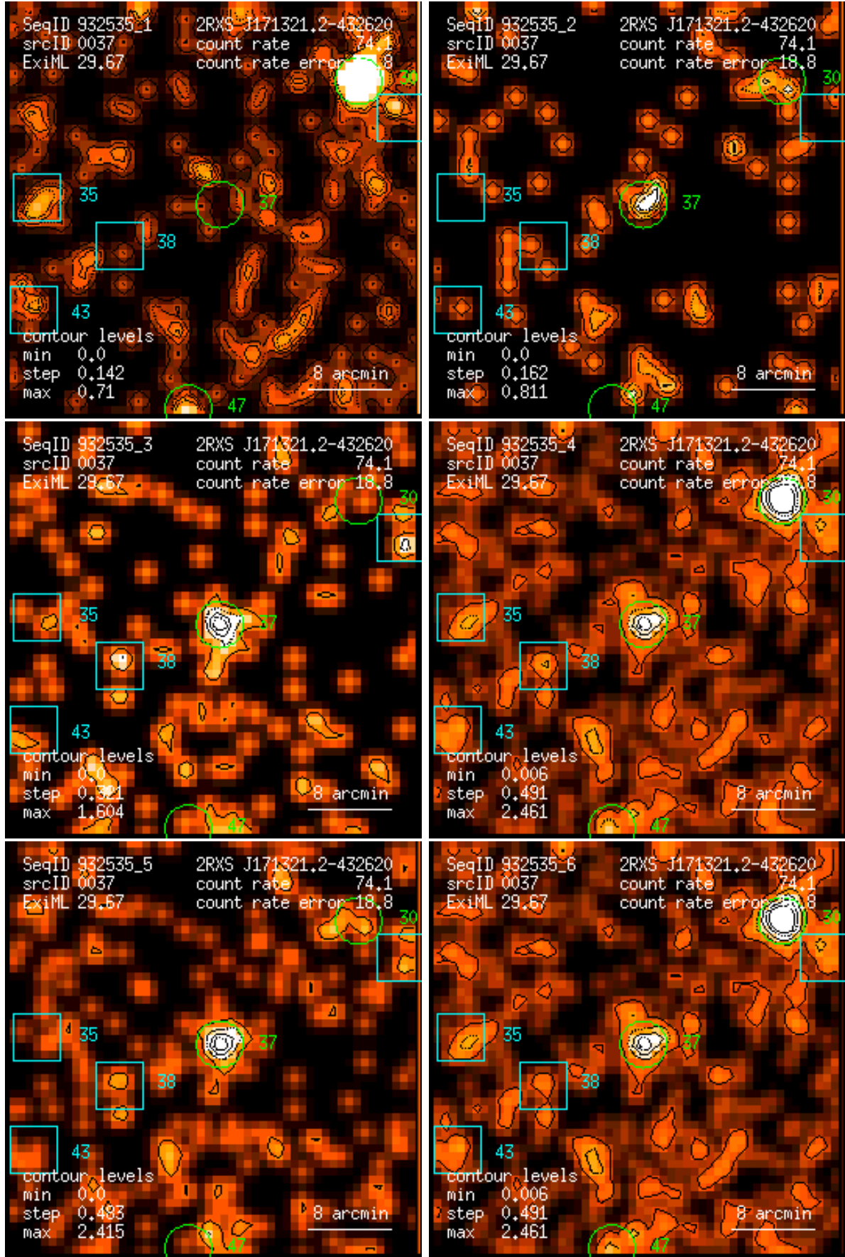
Figure 37: RASS 932535: detection 0037: band rate images, Gaussian filter: (1) PSPC channels 11 – 41, (2) 52 – 90, (3) 91 – 201, (4) 11 – 235, (5) 52 – 201, (6) 11 – 201. Broad band rates in counts/ks. Band rate contour levels in counts/ks/arcmin 2 .
