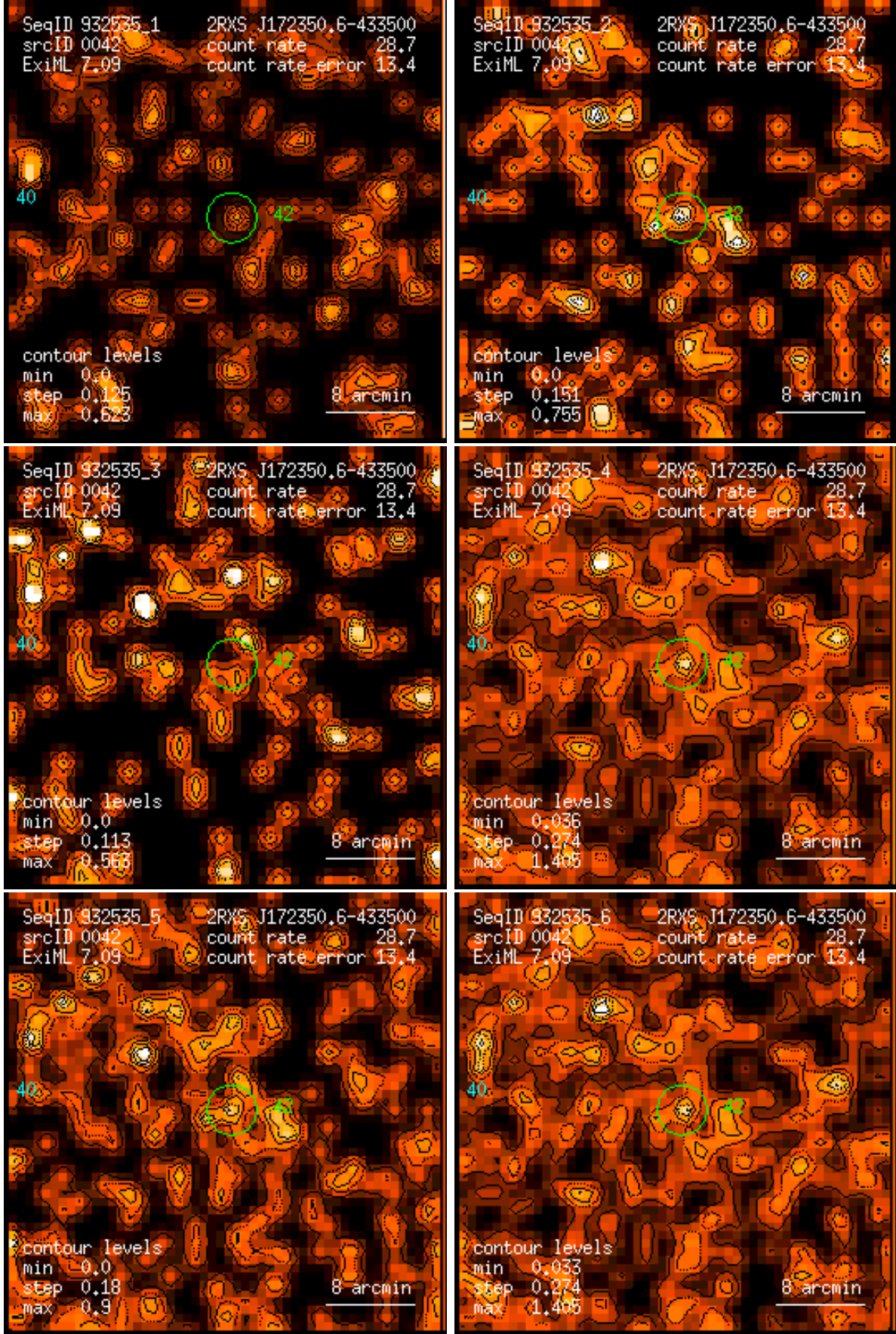
Figure 42: RASS 932535: detection 0042: band rate images, Gaussian filter: (1) PSPC channels 11 – 41, (2) 52 – 90, (3) 91 – 201, (4) 11 – 235, (5) 52 – 201, (6) 11 – 201. Broad band rates in counts/ks. Band rate contour levels in counts/ks/arcmin 2 .
