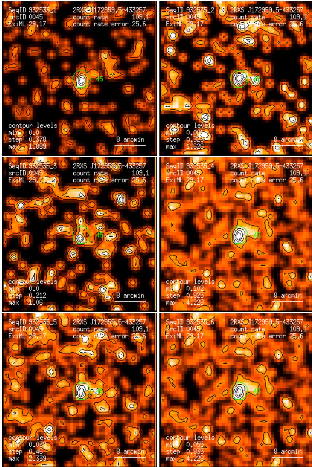
Figure 45: RASS 932535: detection 0045: band rate images, Gaussian filter: (1) PSPC channels 11 – 41, (2) 52 – 90, (3) 91 – 201, (4) 11 – 235, (5) 52 – 201, (6) 11 – 201. Broad band rates in counts/ks. Band rate contour levels in counts/ks/arcmin 2 .
