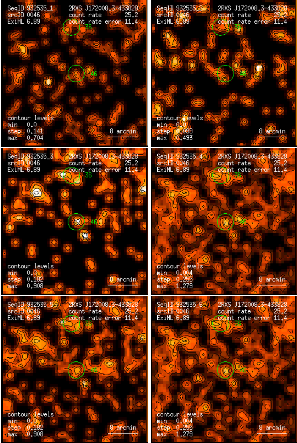
Figure 46: RASS 932535: detection 0046: band rate images, Gaussian filter: (1) PSPC channels 11 – 41, (2) 52 – 90, (3) 91 – 201, (4) 11 – 235, (5) 52 – 201, (6) 11 – 201. Broad band rates in counts/ks. Band rate contour levels in counts/ks/arcmin 2 .
