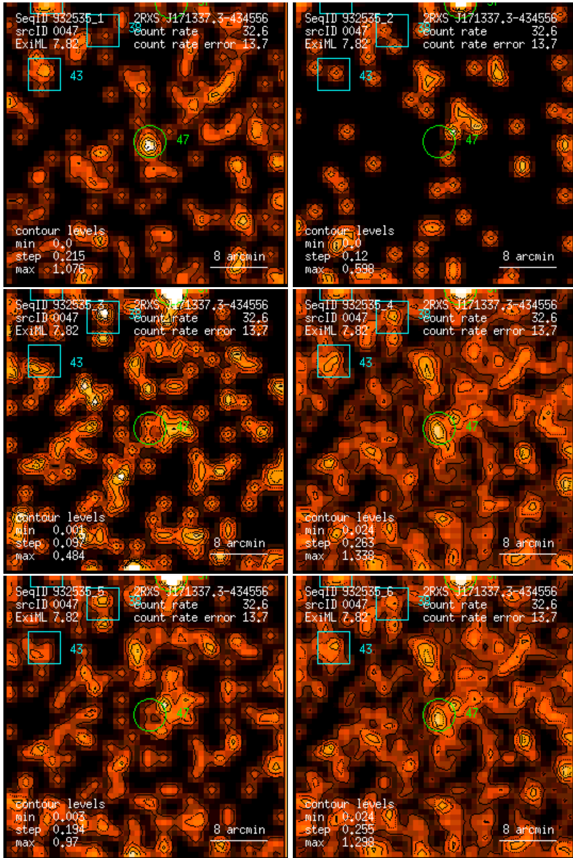
Figure 47: RASS 932535: detection 0047: band rate images, Gaussian filter: (1) PSPC channels 11 – 41, (2) 52 – 90, (3) 91 – 201, (4) 11 – 235, (5) 52 – 201, (6) 11 – 201. Broad band rates in counts/ks. Band rate contour levels in counts/ks/arcmin 2 .
