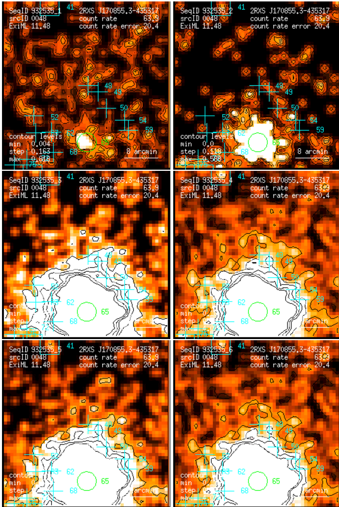
Figure 48: RASS 932535: detection 0048: band rate images, Gaussian filter: (1) PSPC channels 11 – 41, (2) 52 – 90, (3) 91 – 201, (4) 11 – 235, (5) 52 – 201, (6) 11 – 201. Broad band rates in counts/ks. Band rate contour levels in counts/ks/arcmin 2 .
