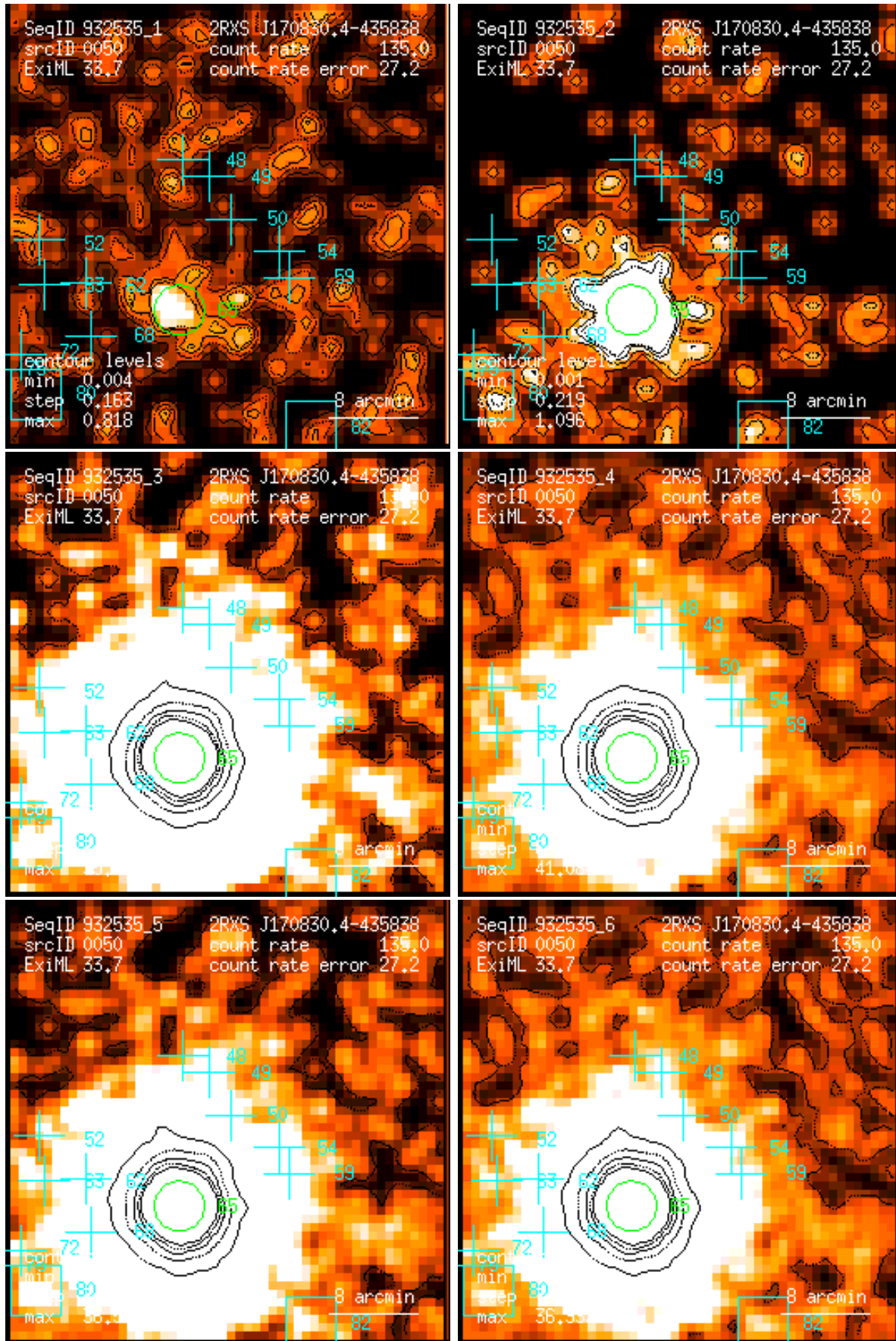
Figure 50: RASS 932535: detection 0050: band rate images, Gaussian filter: (1) PSPC channels 11 – 41, (2) 52 – 90, (3) 91 – 201, (4) 11 – 235, (5) 52 – 201, (6) 11 – 201. Broad band rates in counts/ks. Band rate contour levels in counts/ks/arcmin 2 .
