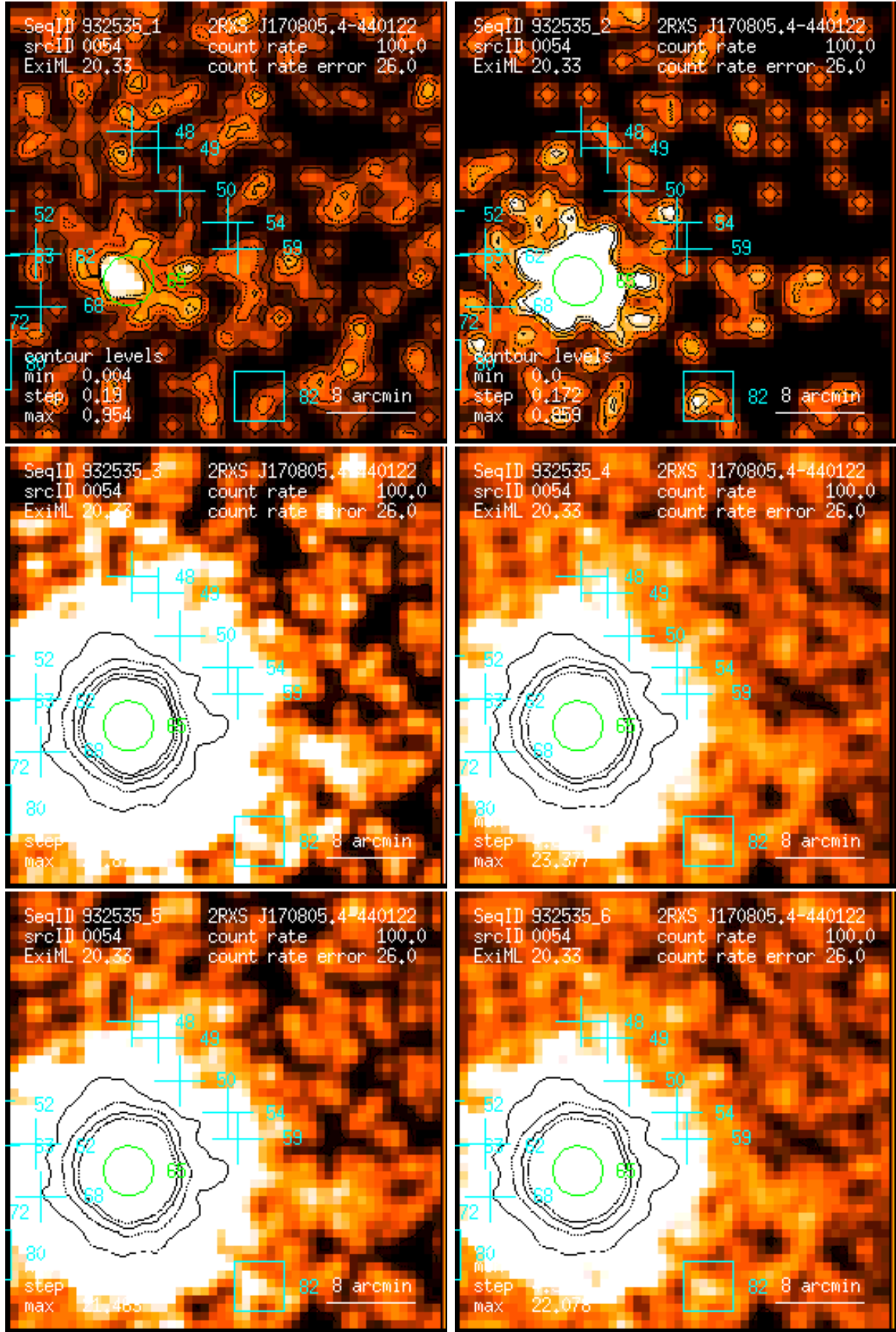
Figure 54: RASS 932535: detection 0054: band rate images, Gaussian filter: (1) PSPC channels 11 – 41, (2) 52 – 90, (3) 91 – 201, (4) 11 – 235, (5) 52 – 201, (6) 11 – 201. Broad band rates in counts/ks. Band rate contour levels in counts/ks/arcmin 2 .
