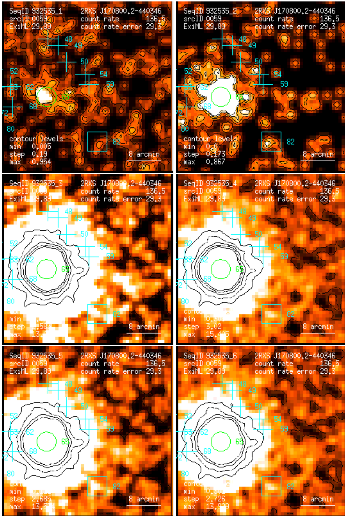
Figure 59: RASS 932535: detection 0059: band rate images, Gaussian filter: (1) PSPC channels 11 – 41, (2) 52 – 90, (3) 91 – 201, (4) 11 – 235, (5) 52 – 201, (6) 11 – 201. Broad band rates in counts/ks. Band rate contour levels in counts/ks/arcmin 2 .
