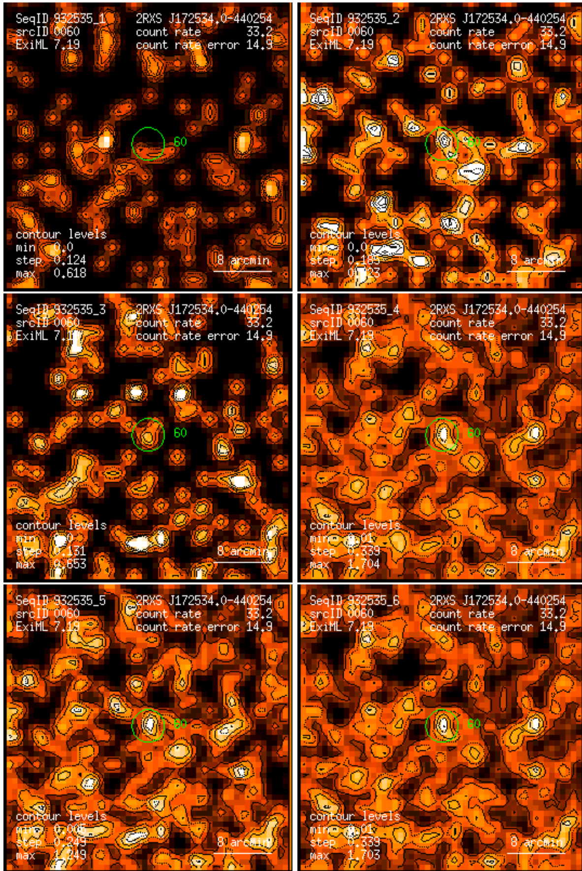
Figure 60: RASS 932535: detection 0060: band rate images, Gaussian filter: (1) PSPC channels 11 – 41, (2) 52 – 90, (3) 91 – 201, (4) 11 – 235, (5) 52 – 201, (6) 11 – 201. Broad band rates in counts/ks. Band rate contour levels in counts/ks/arcmin 2 .
