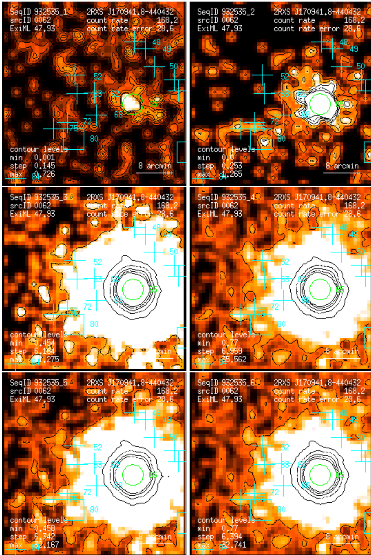
Figure 62: RASS 932535: detection 0062: band rate images, Gaussian filter: (1) PSPC channels 11 – 41, (2) 52 – 90, (3) 91 – 201, (4) 11 – 235, (5) 52 – 201, (6) 11 – 201. Broad band rates in counts/ks. Band rate contour levels in counts/ks/arcmin 2 .
