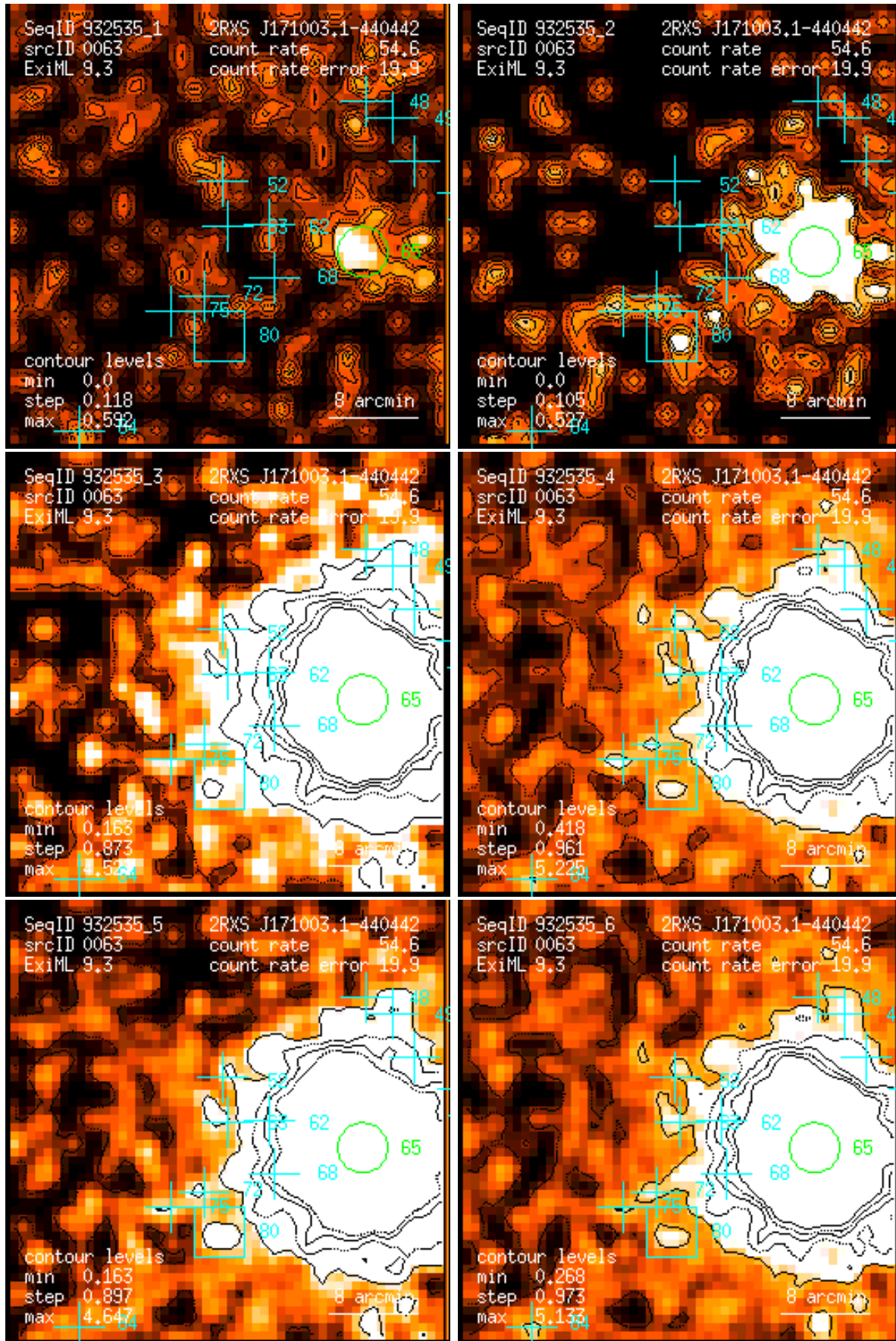
Figure 63: RASS 932535: detection 0063: band rate images, Gaussian filter: (1) PSPC channels 11 – 41, (2) 52 – 90, (3) 91 – 201, (4) 11 – 235, (5) 52 – 201, (6) 11 – 201. Broad band rates in counts/ks. Band rate contour levels in counts/ks/arcmin 2 .
