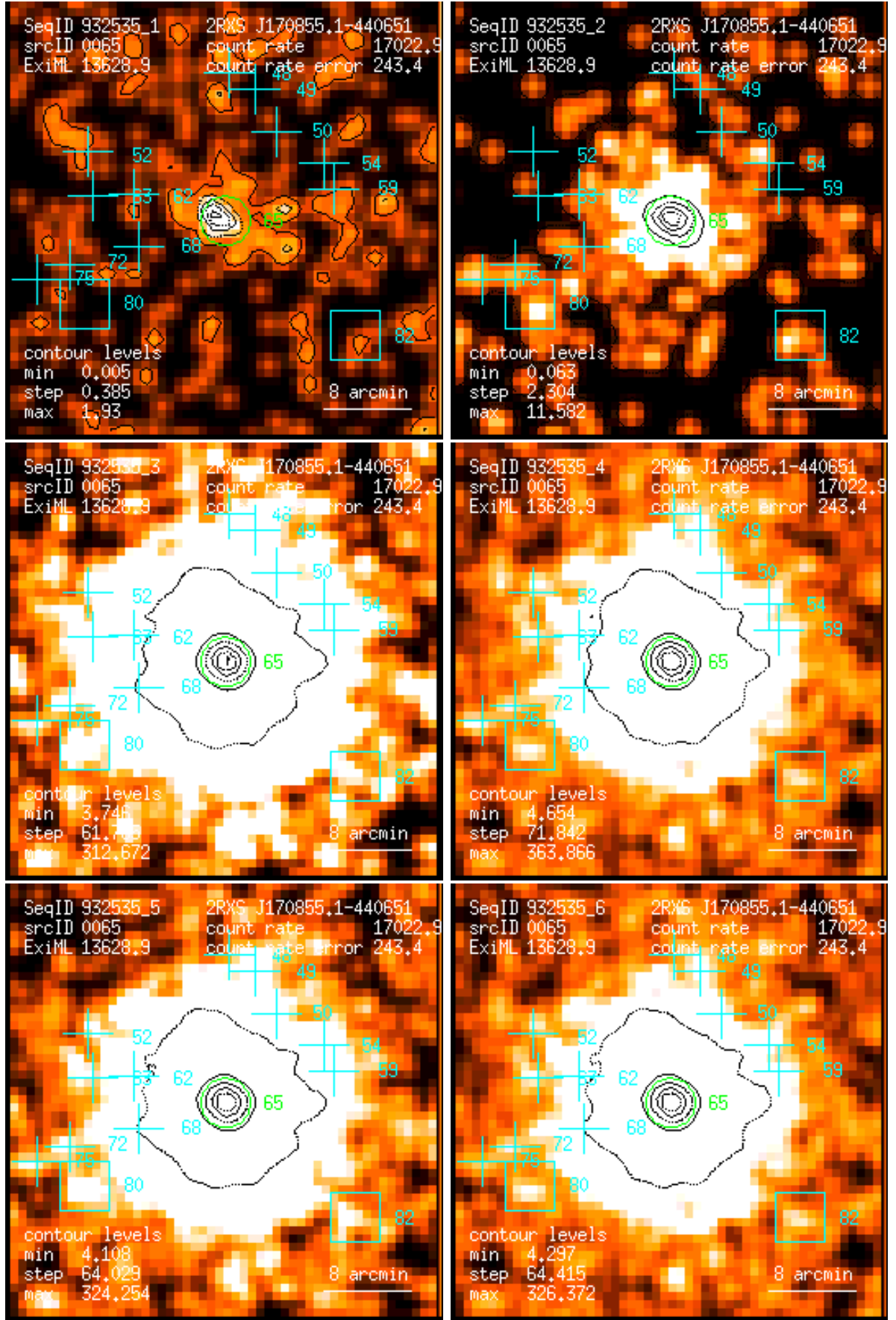
Figure 65: RASS 932535: detection 0065: band rate images, Gaussian filter: (1) PSPC channels 11 – 41, (2) 52 – 90, (3) 91 – 201, (4) 11 – 235, (5) 52 – 201, (6) 11 – 201. Broad band rates in counts/ks. Band rate contour levels in counts/ks/arcmin 2 .
