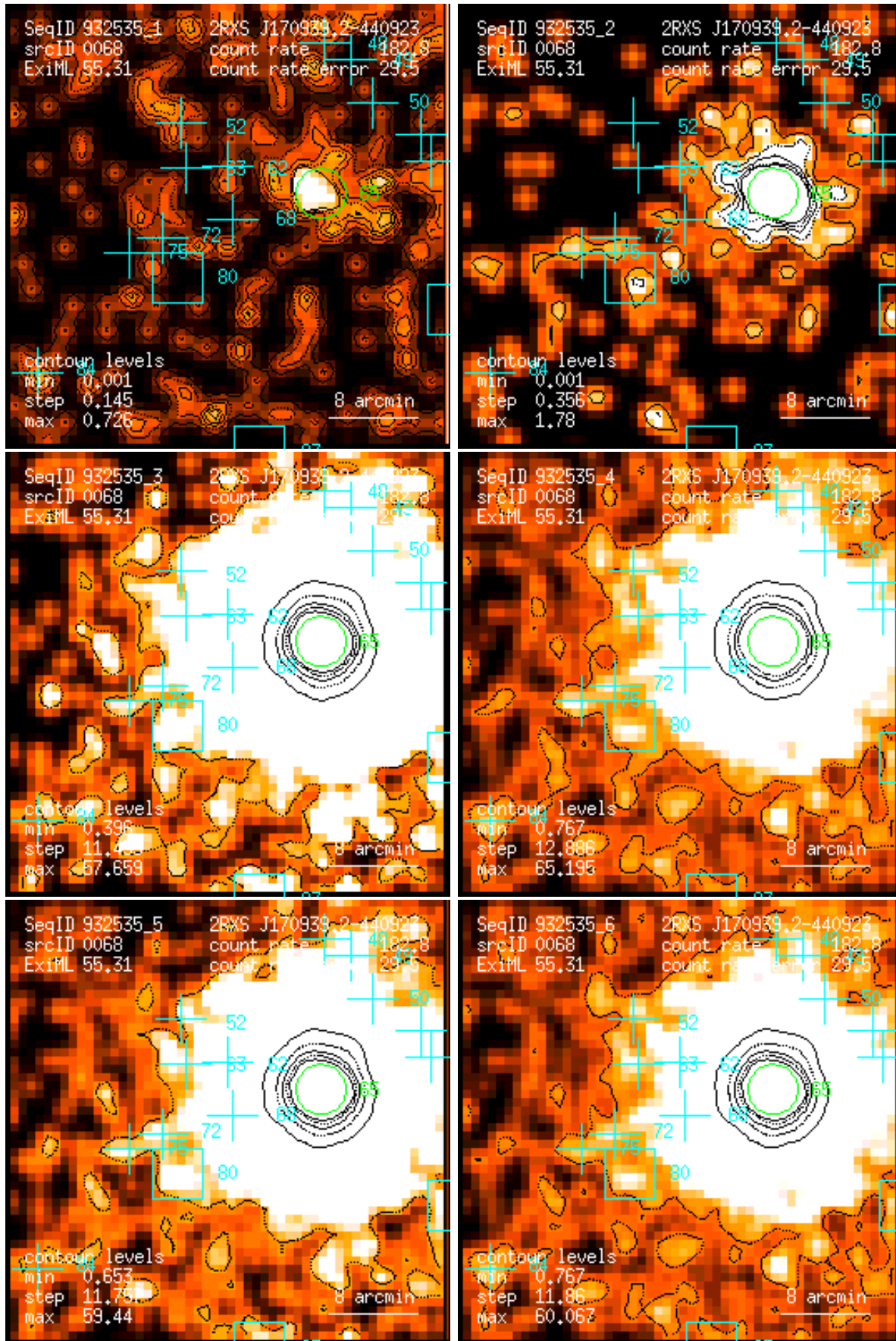
Figure 68: RASS 932535: detection 0068: band rate images, Gaussian filter: (1) PSPC channels 11 – 41, (2) 52 – 90, (3) 91 – 201, (4) 11 – 235, (5) 52 – 201, (6) 11 – 201. Broad band rates in counts/ks. Band rate contour levels in counts/ks/arcmin 2 .
