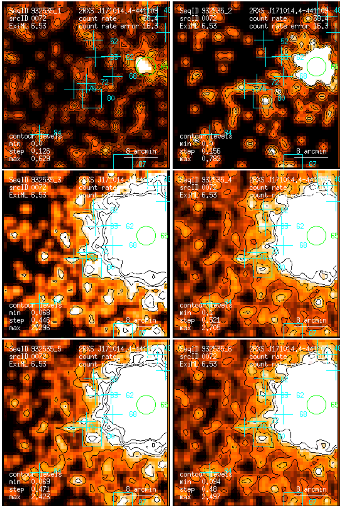
Figure 72: RASS 932535: detection 0072: band rate images, Gaussian filter: (1) PSPC channels 11 – 41, (2) 52 – 90, (3) 91 – 201, (4) 11 – 235, (5) 52 – 201, (6) 11 – 201. Broad band rates in counts/ks. Band rate contour levels in counts/ks/arcmin 2 .
