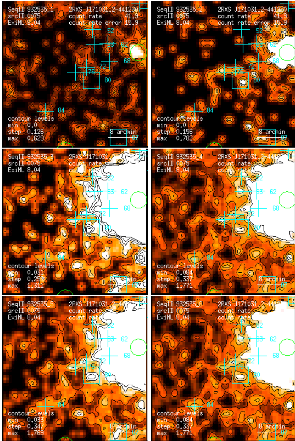
Figure 75: RASS 932535: detection 0075: band rate images, Gaussian filter: (1) PSPC channels 11 – 41, (2) 52 – 90, (3) 91 – 201, (4) 11 – 235, (5) 52 – 201, (6) 11 – 201. Broad band rates in counts/ks. Band rate contour levels in counts/ks/arcmin 2 .
