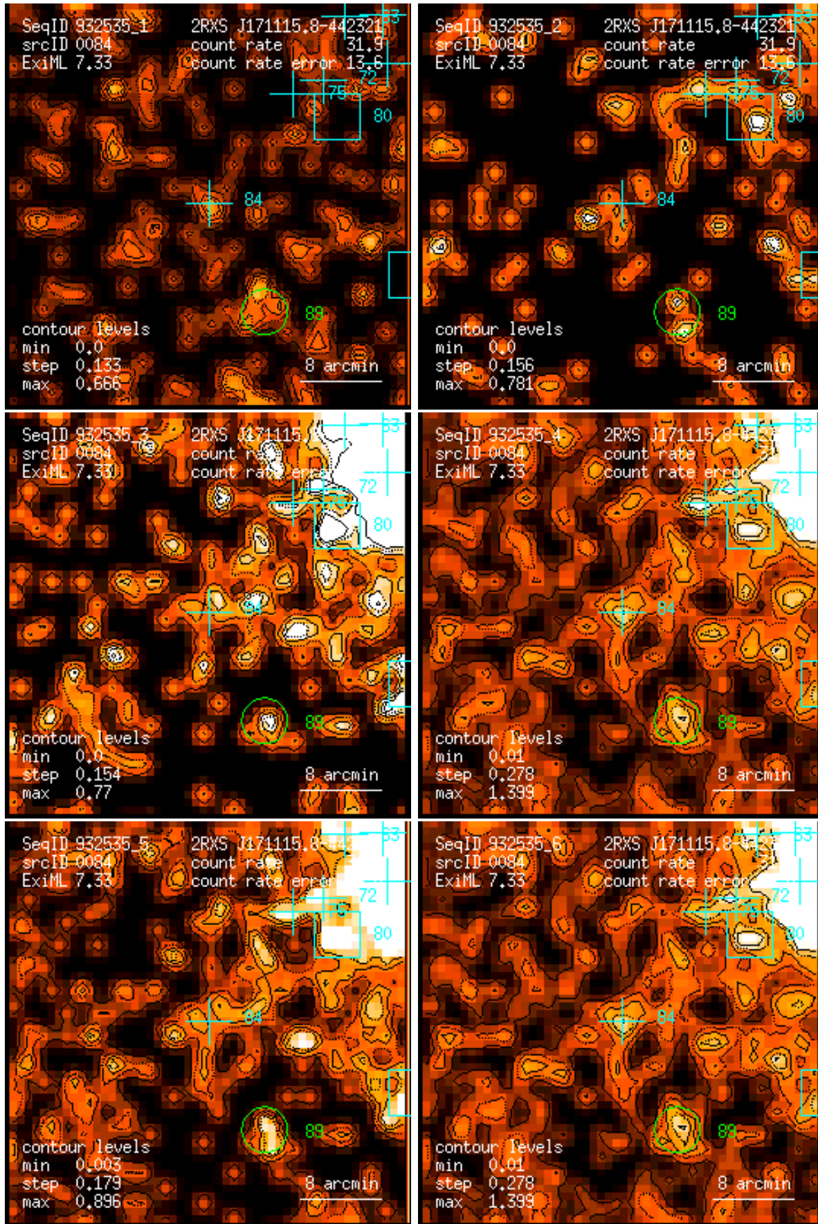
Figure 84: RASS 932535: detection 0084: band rate images, Gaussian filter: (1) PSPC channels 11 – 41, (2) 52 – 90, (3) 91 – 201, (4) 11 – 235, (5) 52 – 201, (6) 11 – 201. Broad band rates in counts/ks. Band rate contour levels in counts/ks/arcmin 2 .
