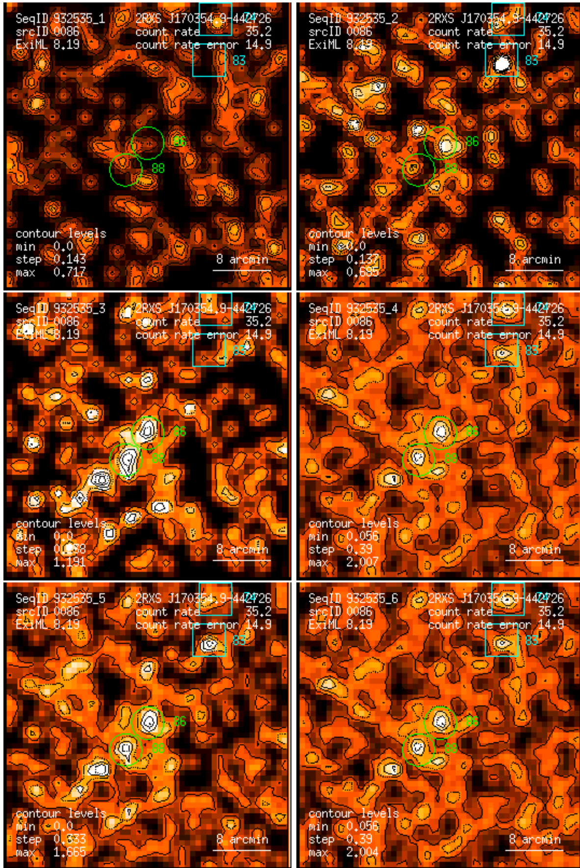
Figure 86: RASS 932535: detection 0086: band rate images, Gaussian filter: (1) PSPC channels 11 – 41, (2) 52 – 90, (3) 91 – 201, (4) 11 – 235, (5) 52 – 201, (6) 11 – 201. Broad band rates in counts/ks. Band rate contour levels in counts/ks/arcmin 2 .
