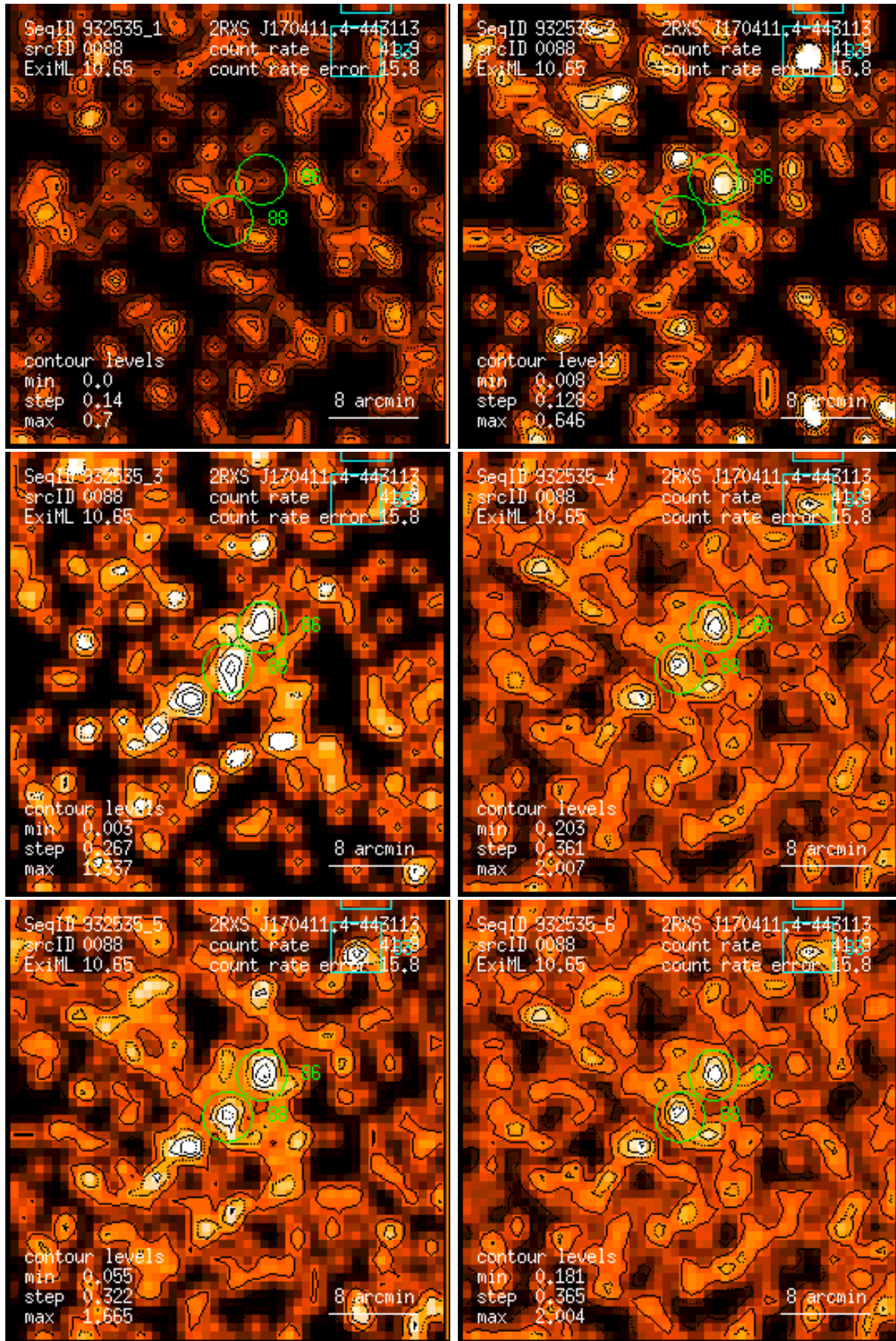
Figure 88: RASS 932535: detection 0088: band rate images, Gaussian filter: (1) PSPC channels 11 – 41, (2) 52 – 90, (3) 91 – 201, (4) 11 – 235, (5) 52 – 201, (6) 11 – 201. Broad band rates in counts/ks. Band rate contour levels in counts/ks/arcmin 2 .
