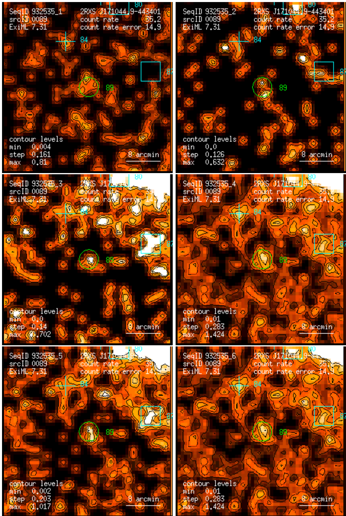
Figure 89: RASS 932535: detection 0089: band rate images, Gaussian filter: (1) PSPC channels 11 – 41, (2) 52 – 90, (3) 91 – 201, (4) 11 – 235, (5) 52 – 201, (6) 11 – 201. Broad band rates in counts/ks. Band rate contour levels in counts/ks/arcmin 2 .
