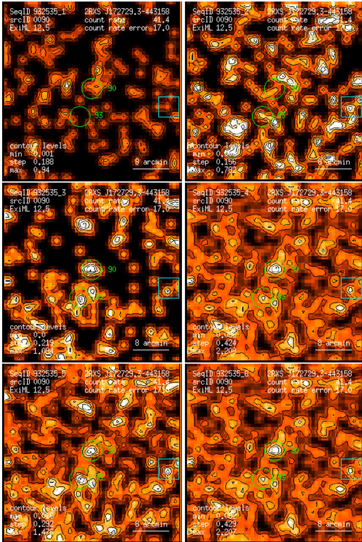
Figure 90: RASS 932535: detection 0090: band rate images, Gaussian filter: (1) PSPC channels 11 – 41, (2) 52 – 90, (3) 91 – 201, (4) 11 – 235, (5) 52 – 201, (6) 11 – 201. Broad band rates in counts/ks. Band rate contour levels in counts/ks/arcmin 2 .
