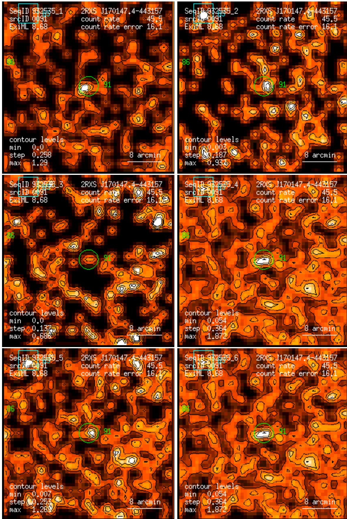
Figure 91: RASS 932535: detection 0091: band rate images, Gaussian filter: (1) PSPC channels 11 – 41, (2) 52 – 90, (3) 91 – 201, (4) 11 – 235, (5) 52 – 201, (6) 11 – 201. Broad band rates in counts/ks. Band rate contour levels in counts/ks/arcmin 2 .
