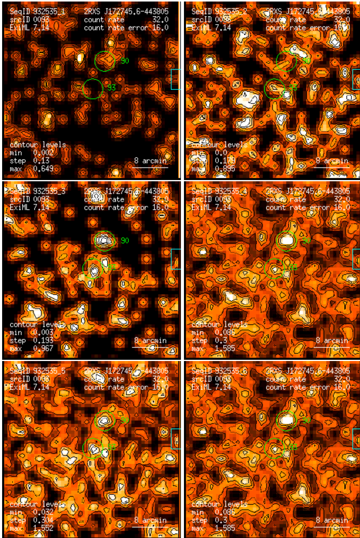
Figure 93: RASS 932535: detection 0093: band rate images, Gaussian filter: (1) PSPC channels 11 – 41, (2) 52 – 90, (3) 91 – 201, (4) 11 – 235, (5) 52 – 201, (6) 11 – 201. Broad band rates in counts/ks. Band rate contour levels in counts/ks/arcmin 2 .
