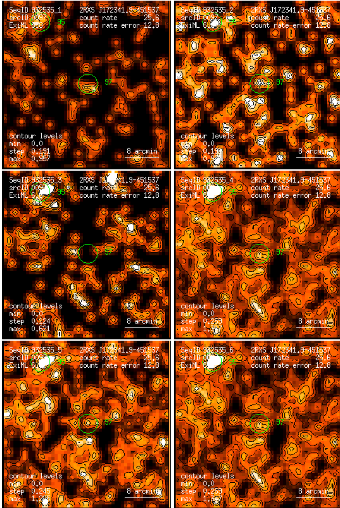
Figure 97: RASS 932535: detection 0097: band rate images, Gaussian filter: (1) PSPC channels 11 – 41, (2) 52 – 90, (3) 91 – 201, (4) 11 – 235, (5) 52 – 201, (6) 11 – 201. Broad band rates in counts/ks. Band rate contour levels in counts/ks/arcmin 2 .
