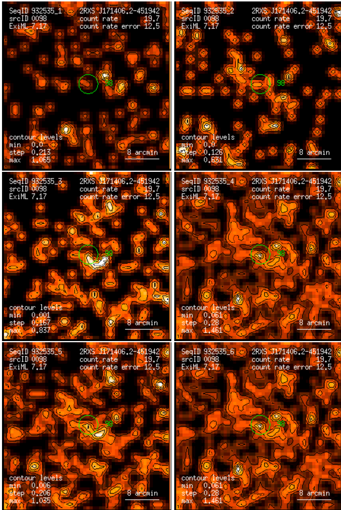
Figure 98: RASS 932535: detection 0098: band rate images, Gaussian filter: (1) PSPC channels 11 – 41, (2) 52 – 90, (3) 91 – 201, (4) 11 – 235, (5) 52 – 201, (6) 11 – 201. Broad band rates in counts/ks. Band rate contour levels in counts/ks/arcmin 2 .
