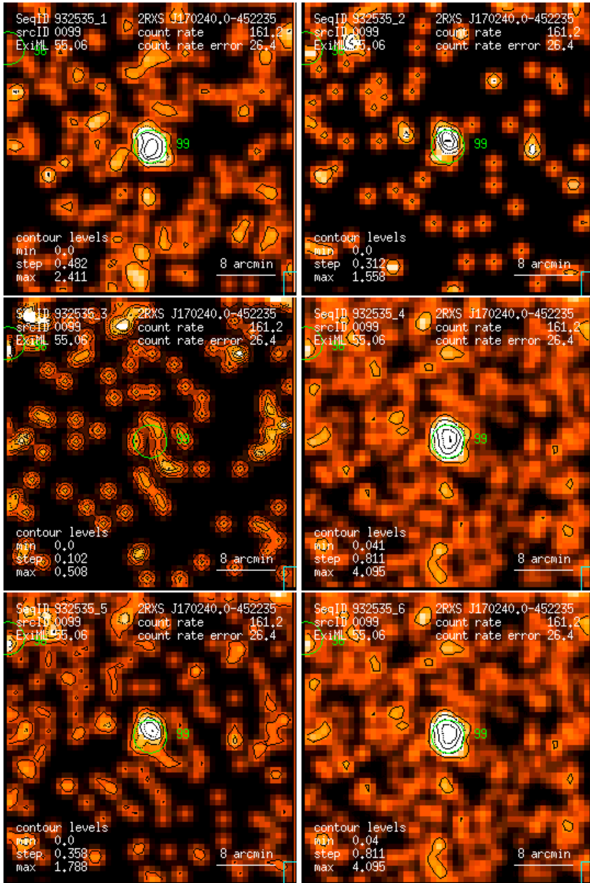
Figure 99: RASS 932535: detection 0099: band rate images, Gaussian filter: (1) PSPC channels 11 – 41, (2) 52 – 90, (3) 91 – 201, (4) 11 – 235, (5) 52 – 201, (6) 11 – 201. Broad band rates in counts/ks. Band rate contour levels in counts/ks/arcmin 2 .
