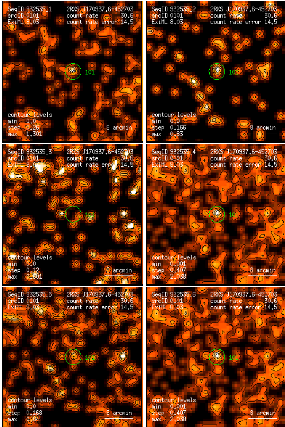
Figure 101: RASS 932535: detection 0101: band rate images, Gaussian filter: (1) PSPC channels 11 – 41, (2) 52 – 90, (3) 91 – 201, (4) 11 – 235, (5) 52 – 201, (6) 11 – 201. Broad band rates in counts/ks. Band rate contour levels in counts/ks/arcmin 2 .
