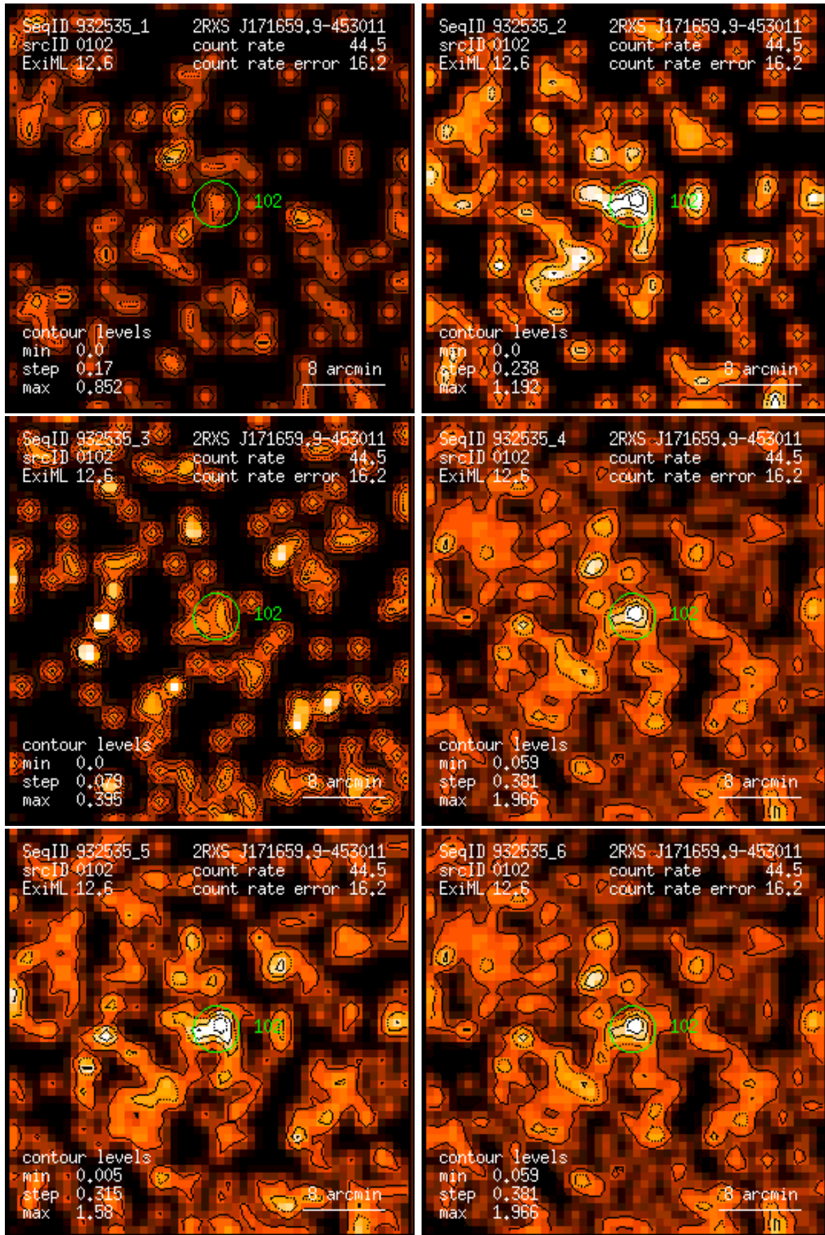
Figure 102: RASS 932535: detection 0102: band rate images, Gaussian filter: (1) PSPC channels 11 – 41, (2) 52 – 90, (3) 91 – 201, (4) 11 – 235, (5) 52 – 201, (6) 11 – 201. Broad band rates in counts/ks. Band rate contour levels in counts/ks/arcmin 2 .
