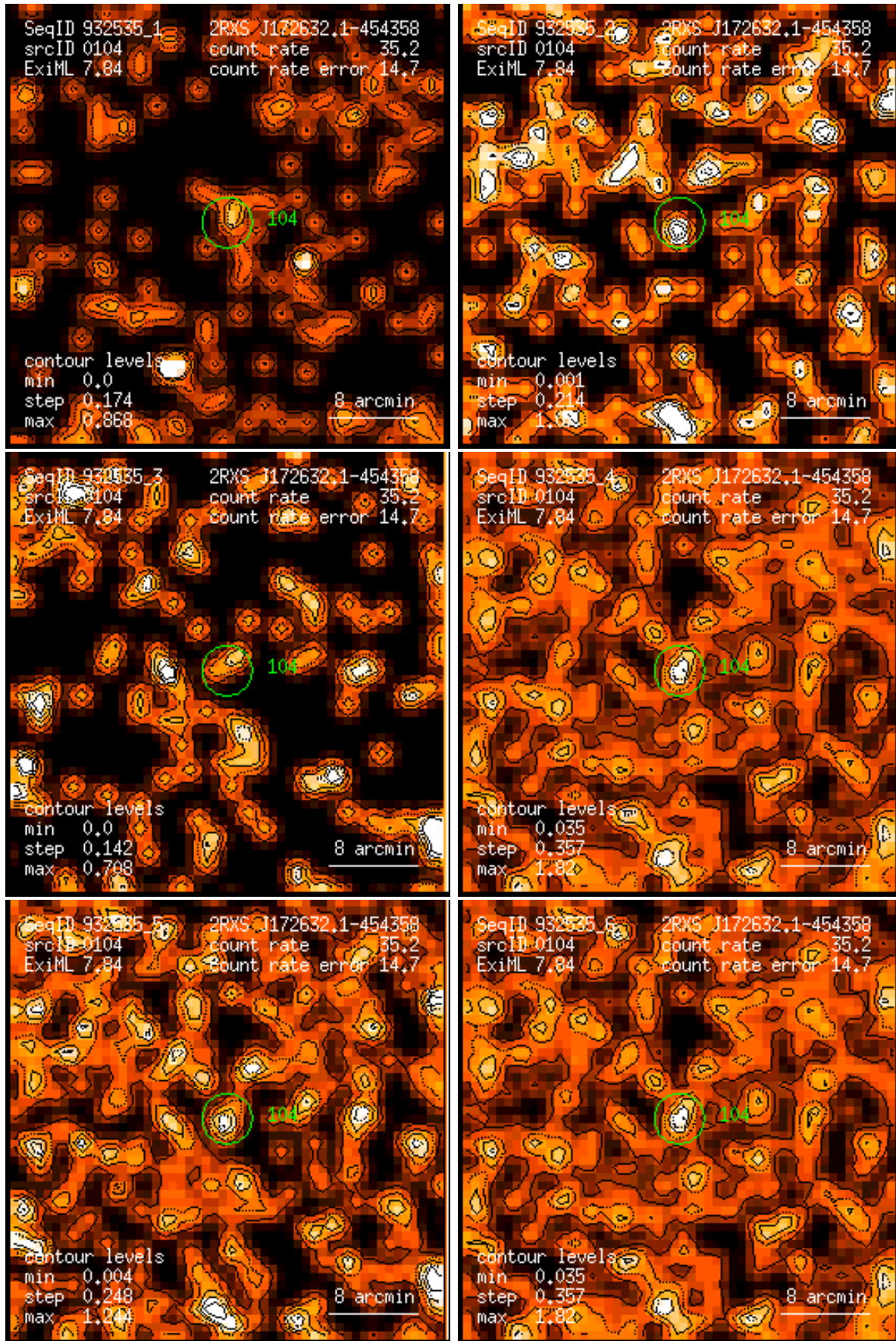
Figure 104: RASS 932535: detection 0104: band rate images, Gaussian filter: (1) PSPC channels 11 – 41, (2) 52 – 90, (3) 91 – 201, (4) 11 – 235, (5) 52 – 201, (6) 11 – 201. Broad band rates in counts/ks. Band rate contour levels in counts/ks/arcmin 2 .
