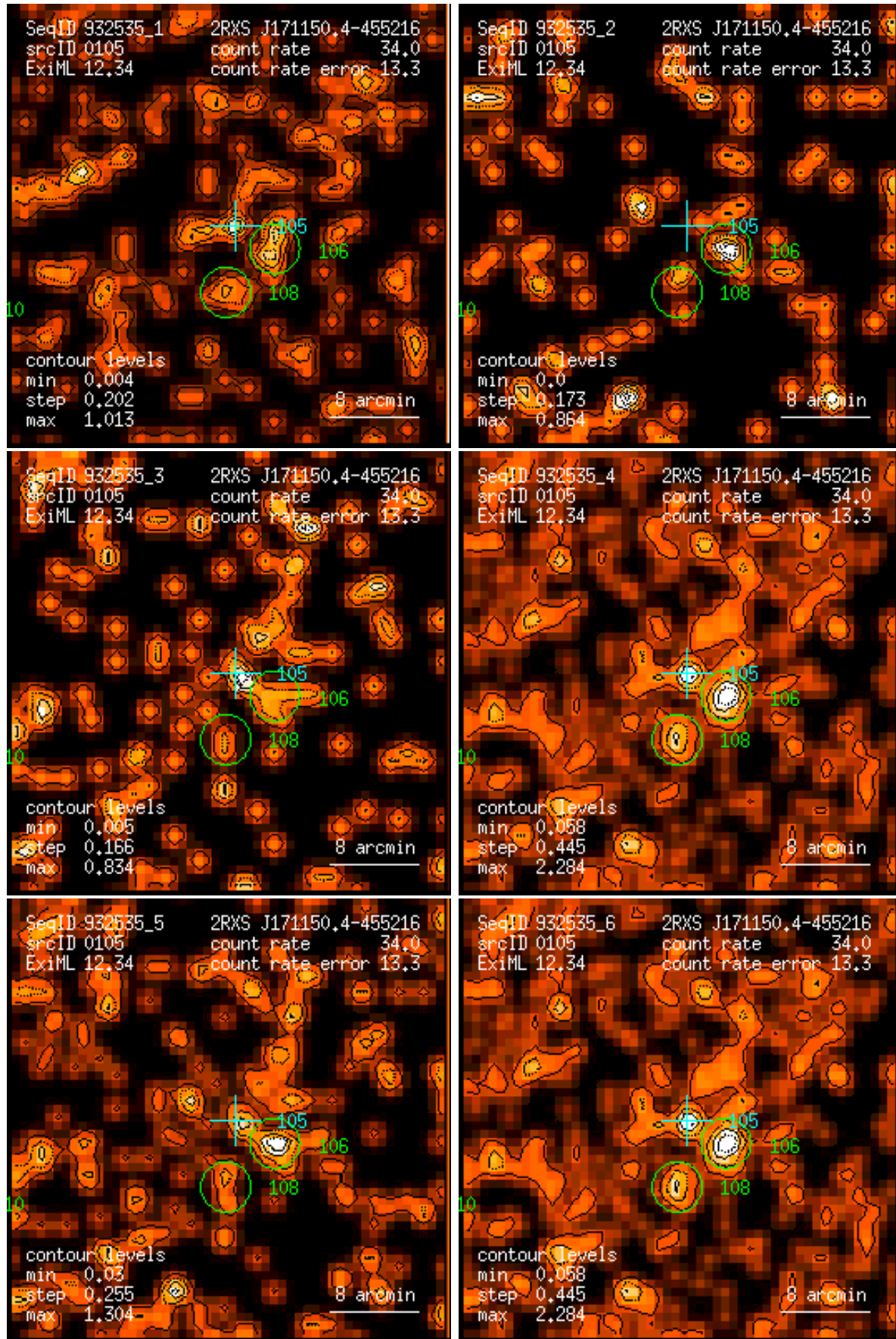
Figure 105: RASS 932535: detection 0105: band rate images, Gaussian filter: (1) PSPC channels 11 – 41, (2) 52 – 90, (3) 91 – 201, (4) 11 – 235, (5) 52 – 201, (6) 11 – 201. Broad band rates in counts/ks. Band rate contour levels in counts/ks/arcmin 2 .
