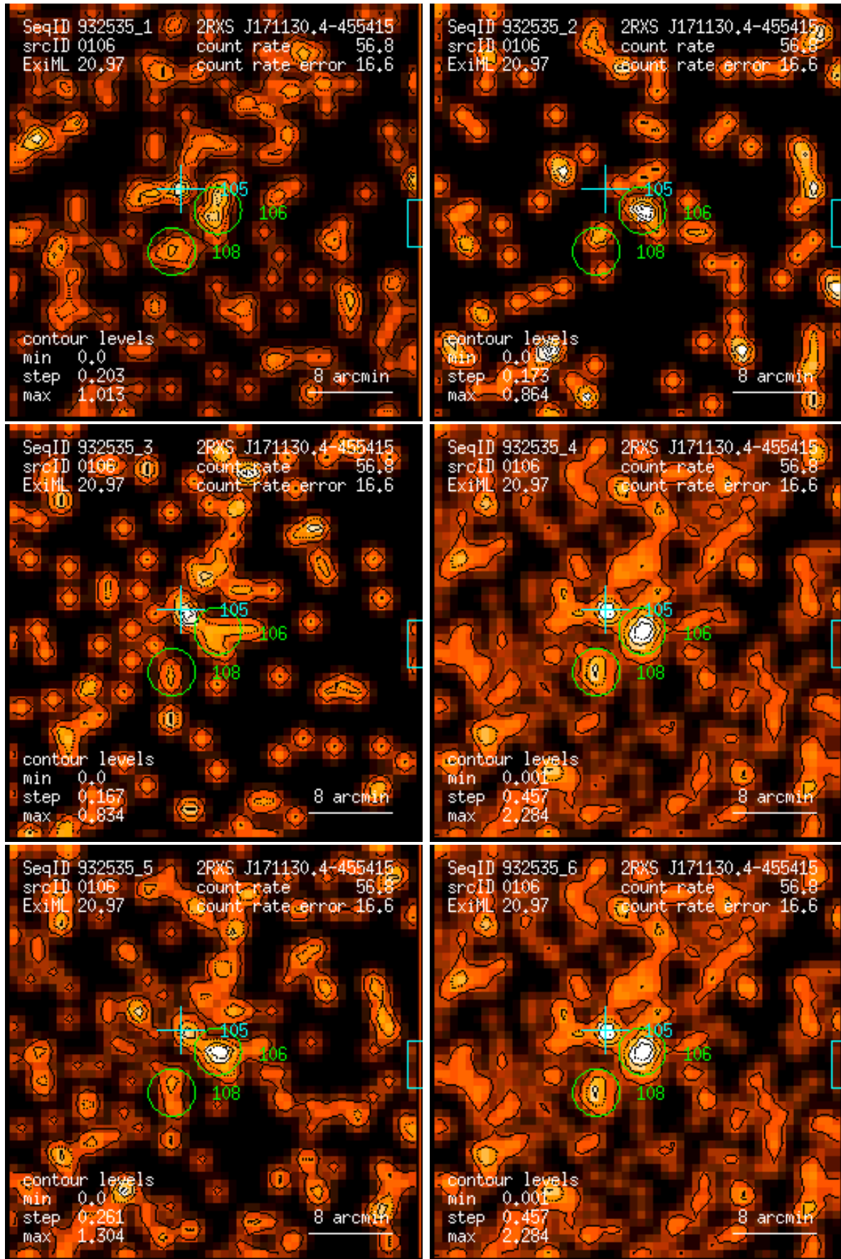
Figure 106: RASS 932535: detection 0106: band rate images, Gaussian filter: (1) PSPC channels 11 – 41, (2) 52 – 90, (3) 91 – 201, (4) 11 – 235, (5) 52 – 201, (6) 11 – 201. Broad band rates in counts/ks. Band rate contour levels in counts/ks/arcmin 2 .
