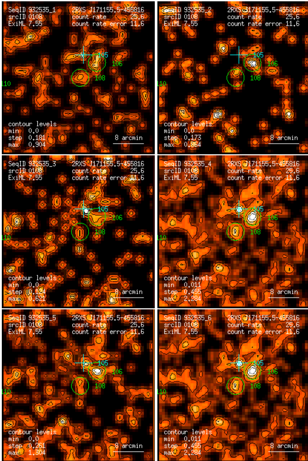
Figure 108: RASS 932535: detection 0108: band rate images, Gaussian filter: (1) PSPC channels 11 – 41, (2) 52 – 90, (3) 91 – 201, (4) 11 – 235, (5) 52 – 201, (6) 11 – 201. Broad band rates in counts/ks. Band rate contour levels in counts/ks/arcmin 2 .
