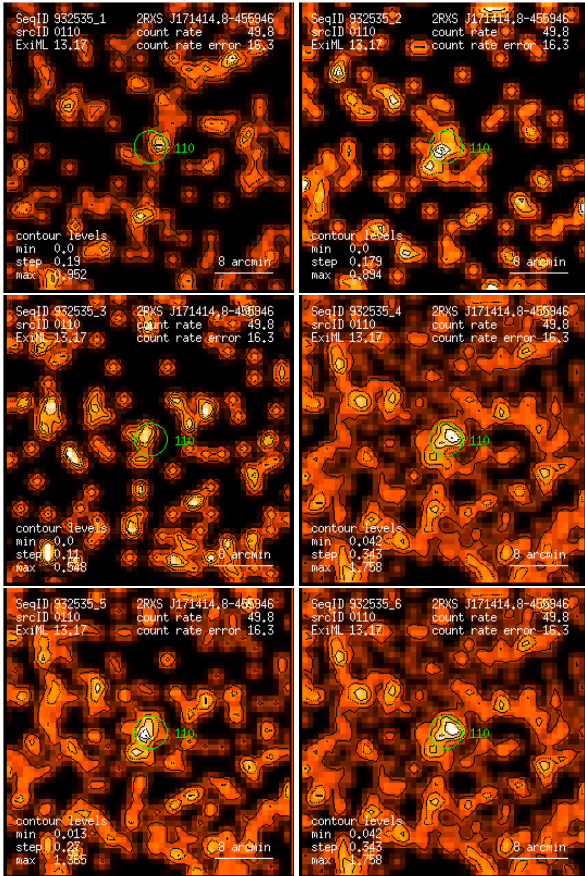
Figure 110: RASS 932535: detection 0110: band rate images, Gaussian filter: (1) PSPC channels 11 – 41, (2) 52 – 90, (3) 91 – 201, (4) 11 – 235, (5) 52 – 201, (6) 11 – 201. Broad band rates in counts/ks. Band rate contour levels in counts/ks/arcmin 2 .
